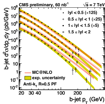
Figure 3: Differential b-jet cross-section. The band indicates the quadratic sum of statistical and systematic uncertainties, not including the luminosity uncertainty. The theoretical prediction from MC@NLO is shown with the lines.
