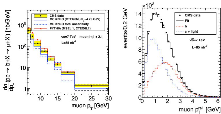
Figure 2: Left: The differential cross-section. The theoretical prediction from MC@NLO and PYTHIA are shown with the lines. The markers represent data points, the band indicates the quadratic sum of statistical and systematic uncertainties. Right: Distribution of the muon p_T^{rel} for b and c+light flavor templates. The black line shows the result of the likelihood fit, the markers show the data points.
