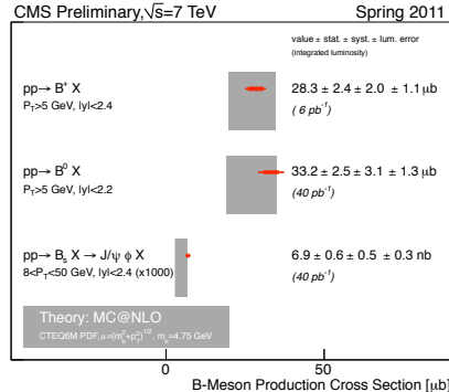
Figure 1: Summary of B meson cross section measurements. The inner error bars of the data points correspond to the statistical uncertainty, the outer error bars correspond to the quadratic sum of statistical and systematic uncertainties. The outermost brackets correspond to the total error, including a luminosity uncertainty.
