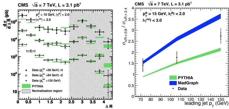
Figure 4: Left: Differential cross-section of B\bar{B} pair production as a function of \Delta R . The PYTHIA simulation (shaded) is normalized to the region \Delta R as indicated by the shaded normalization regions. Right: Ratio between B\bar{B} production cross sections in \Delta R < 0.8 and \Delta R > 2.4 . The predictions from PYTHIA and MadGraph [13] MC generators are also shown. For the data points the inner error bars show statistical uncertainty while the outer ones show the systematic uncertainty
