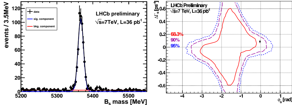
Figure 1: Left: invariant mass distribution of selected B_s^0 \rightarrow J/\psi\phi events. Right: Feldman and Cousins regions in the \Delta\Gamma_s - \phi_s plane. The CL at the SM point (black square) is 0.785 which corresponds to a deviation of 1.2 \sigma .
