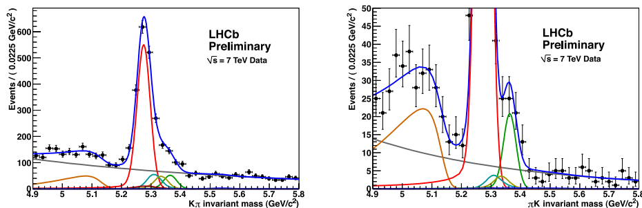
Figure 3: Invariant mass distribution of B^0 \rightarrow K^+\pi^- (left) and B_s^0 \rightarrow \pi^+K^- (right).
