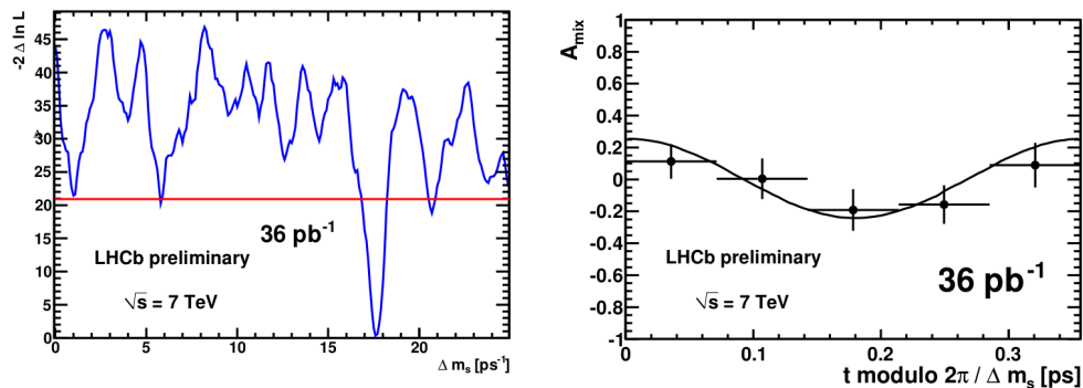
Figure 2: Left: likelihood scan for \Delta m_s the line indicates the likelihood value evaluated in the limit of infinite mixing frequency. Right: mixing asymmetry for signal B_s^0 candidates as a function of decay time modulo 2\pi/\Delta m_s .
