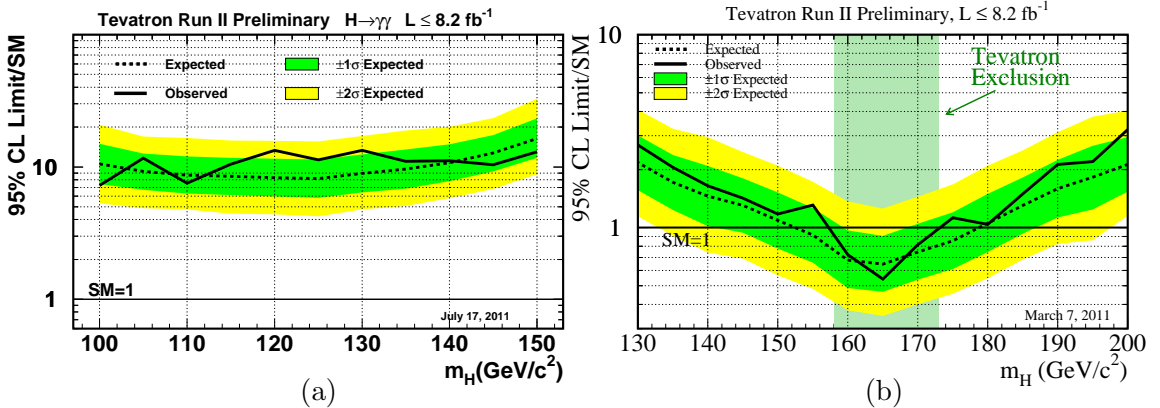
Figure 2: Combined CDF and DØ upper limits on the Standard Model Higgs boson production for the decay channels into two photons (a) and two W bosons (b), where the shaded vertical band represents the excluded mass range.
