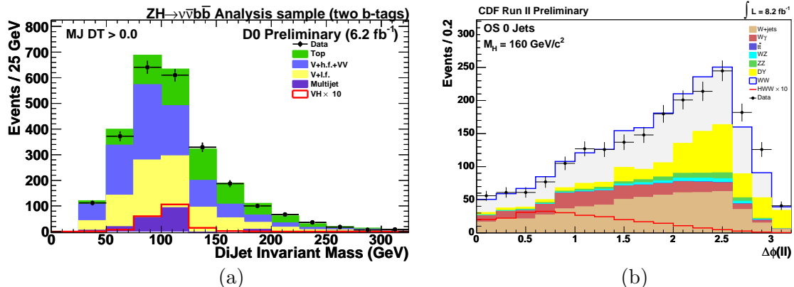
Figure 1: Distributions of the invariant mass of the b -tagged jets in the DØ ZH \rightarrow \nu\bar{\nu}b\bar{b} search (a) and of the \Delta\phi between the leptons from the W decays in the CDF H \rightarrow WW analysis (b) with the expected backgrounds and signal superimposed.
