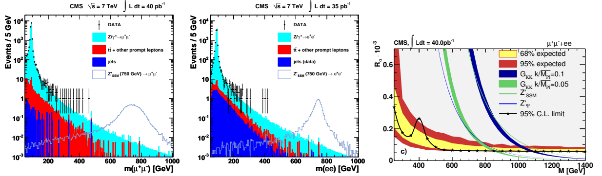
Figure 2: Invariant mass spectrum of \mu^+\mu^- (left) and ee (right) events. The open histogram shows the signal expected for a Z'_{SSM} with a mass of 750 GeV. Upper limits (right) as a function of resonance mass M_{ll} , on the production ratio of \sigma \times BR into lepton pairs for various models.
