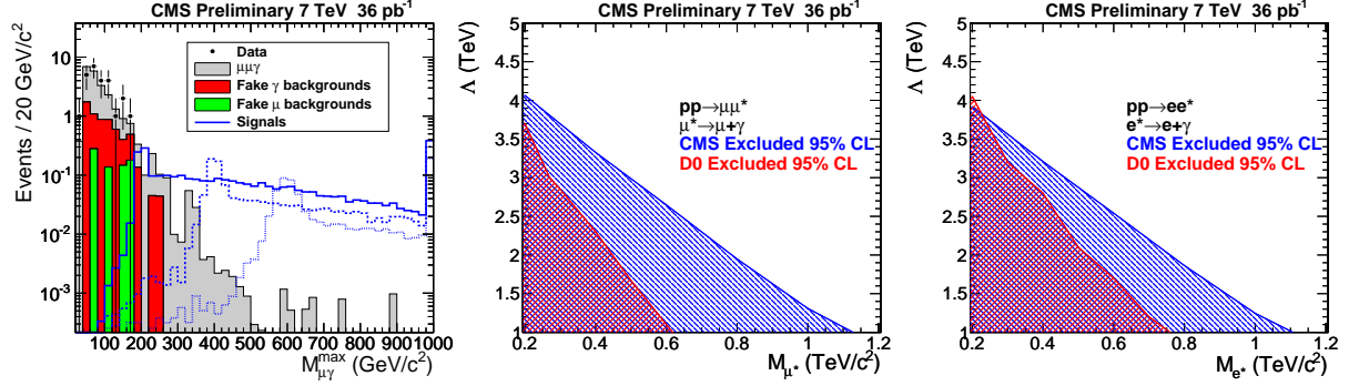
Figure 3: Invariant mass distribution of the chosen l\gamma pair in the muon channel (left). (\Lambda, M_{l^*}) region excluded at the 95% CL, for muons (middle) and electrons (right), compared to previous most stringent limits by the D0 experiment.
