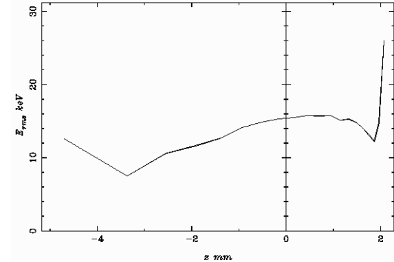
Slice Energy Spread
