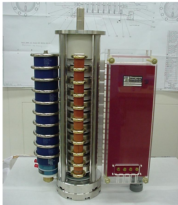
Figure 1: One of two HV switches of an MKD generator: GTO stack (centre), partly hidden behind the voltage distribution resistors; trigger transformer (right); snubber capacitors (left).
