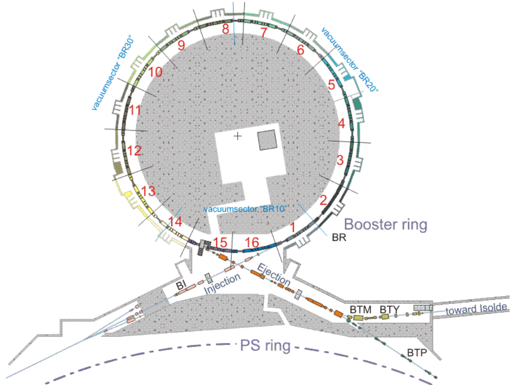
Figure 1: PS Booster and its transfer lines.
