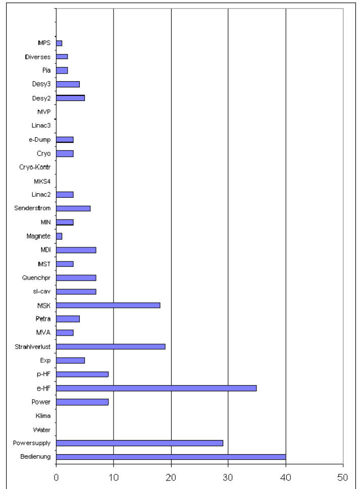
Figure 11: The most frequent reasons for an interruption of the HERA operation in the 2006 run period.
