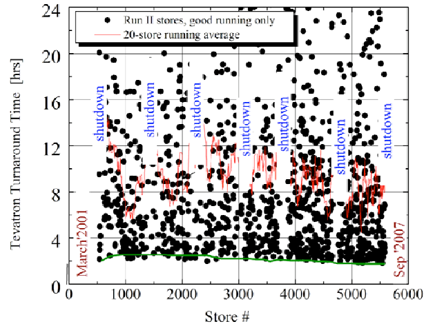
Figure 7: The Tevatron turnaround time as a function of store number with a cut of 36h
