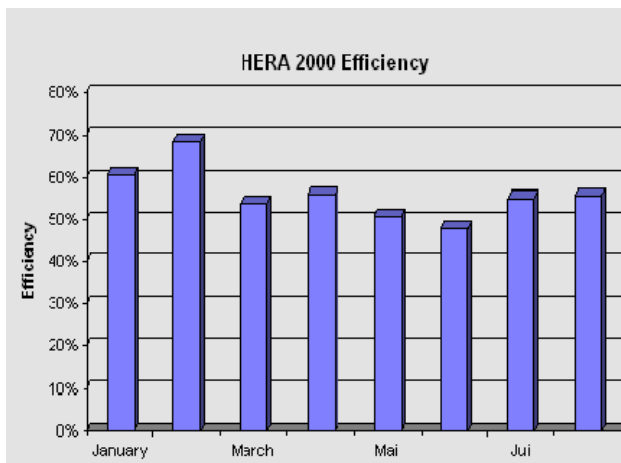
Figure 10: The HERA machine efficiency during the 2000 operation.
