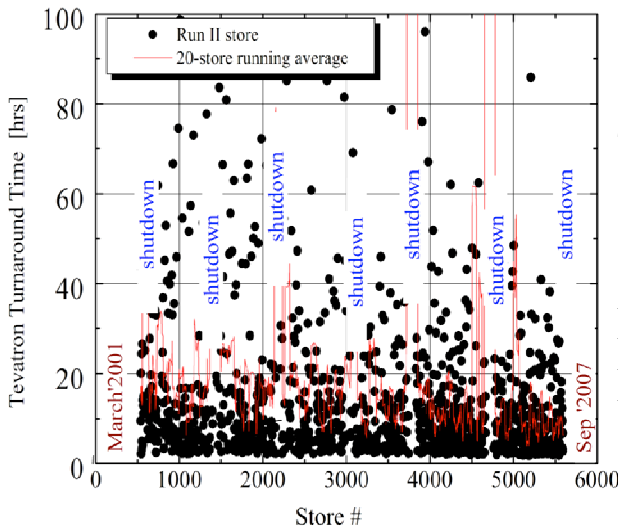
Figure 6: The Tevatron turnaround time as a function of store number.
