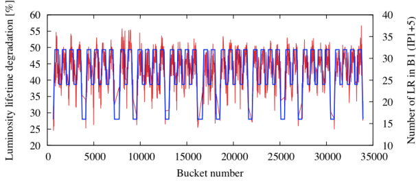
Figure 12: Bunch by bunch luminosity lifetime degradation and number of long range parasitic encounters as a function of the bunch RF bucket. The plots shows a clear dependency of the lifetime degradation with the number of parasitic encounters.
