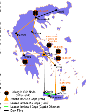
Figure 1 – The GRNET HellasGrid infrastructure
