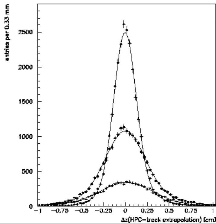
HPC z-resolution
