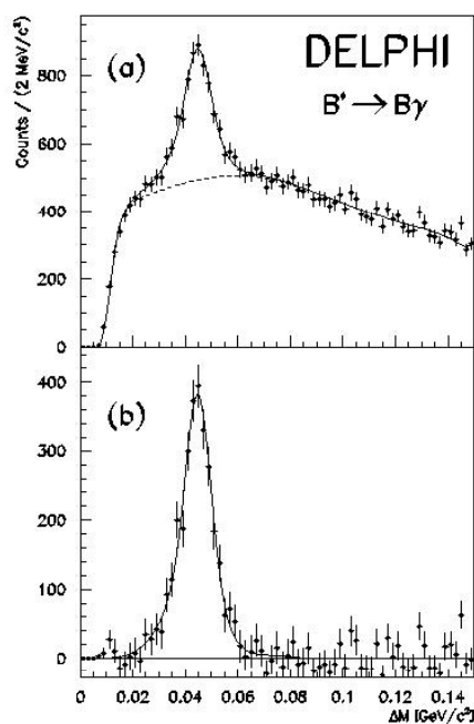
Figure 3: H\gamma - H mass difference distribution. (a) The data are represented by points, the line corresponds to the fit result using background and signal shapes predicted by simulation. (b) The \Delta M(H^* - H) signal after background subtraction. The curve shows the expectation from the simulation with a value of 45.5 \text{ MeV}/c^2 and an isospin splitting of 3.5 \text{ MeV} .
