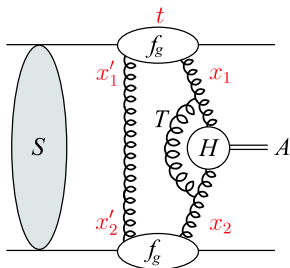
Figure 2: A symbolic diagram for the central exclusive production of a Higgs boson H .
