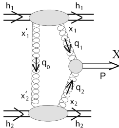
Figure 1: The KKMR mechanism of central exclusive production is similar to Feynman mechanism for form-factors: screening gluon with soft momentum q_0 corresponds to soft quark for form-factor
