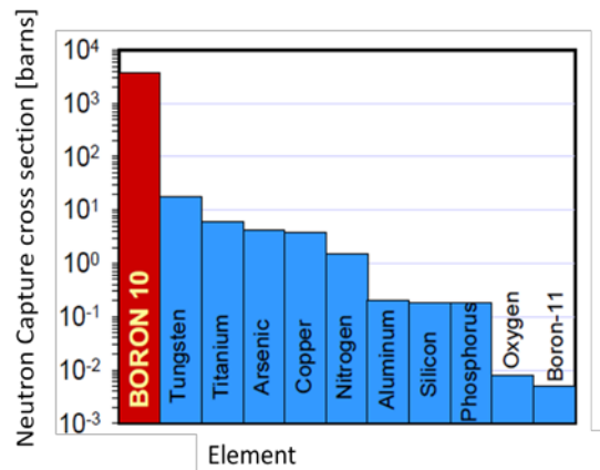
Figure 4: Neutron Capture cross section for various elements that are used in the fabrication of semiconductor devices.
