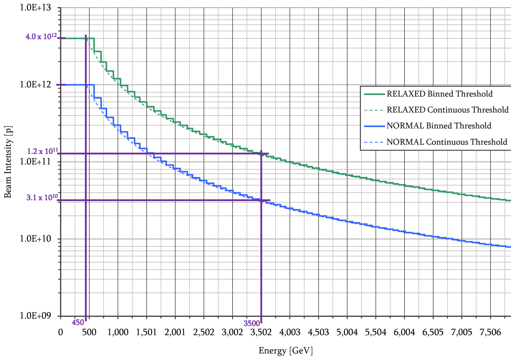
Set-up Beam Flag Transisiton for NORMAL and RELAXED Thresholds
