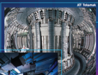
JET Tokamak
