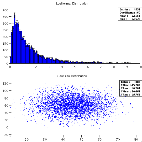
Figure 4: AIDA objects plotted from a C++ program using the Java implementation of the IPlotter interfaces.
