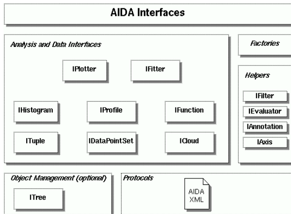
Figure1: The set of AIDA interfaces
