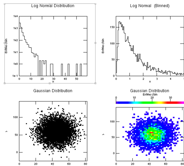
Figure 3: Example of visualization of AIDA objects in HippoDraw
