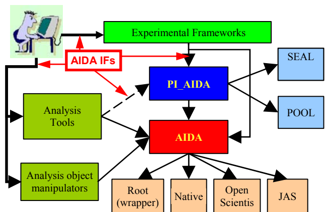
Figure 2: The components of the PI Analysis Systems subsystem (PI_AIDA). The user typically accesses the analysis objects through the experimental framework, an analysis tool, or an analysis object manipulator (e.g., tuple or cloud projector). In all cases, the usage is through the AIDA interfaces (or their PI proxy counterpart), so there is no dependency on the specific implementation at compile or link time.
