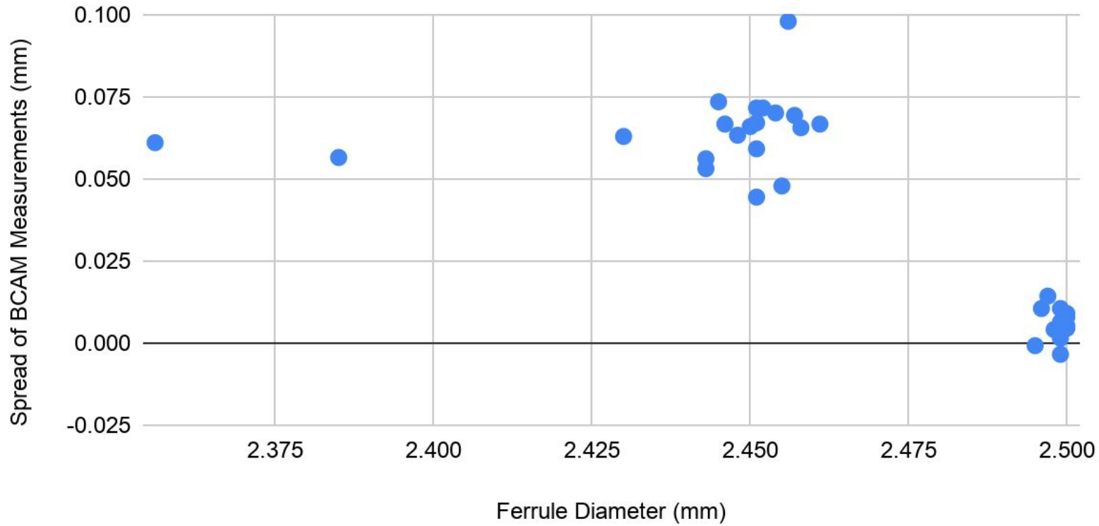
Ferrule Diameter vs. BCAM 50 mm fiber bend measurement
