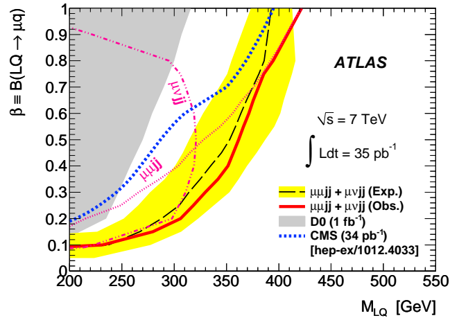
Figure 3: 95% C.L. limits from the muon channel searches on the plane defined by the branching ratio in muon quark of the leptoquarks and their mass.
