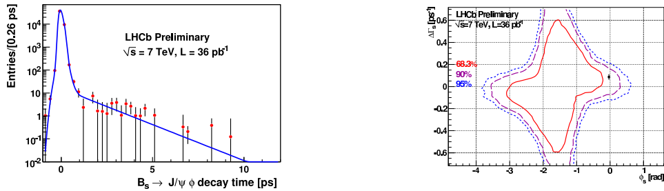
Figure 2: Left: Decay time distribution of background B_s^0 \rightarrow J/\psi\phi candidates obtained with the sPlot [7] technique using the candidate mass as separating observable. The superimposed curve is the background decay time model convolved with the resolution model. The background model includes a prompt component and a long lived component, described by two exponential functions with different decay constants. Right: Feldman-Cousins confidence regions in the \phi_s - \Delta\Gamma_s plane. The CL at the Standard Model point (black square) is 0.785 which corresponds to a deviation of “1.2 \sigma ”.
