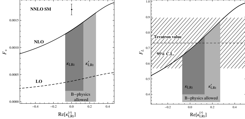
Figure 1: Left: F_+ as a function of \kappa'_{LRt} , LO (dashed) and NLO (solid). Also shown the NNLO SM point with theoretical errors. Right: F_L as a function of \kappa'_{LRt} along with combined Tevatron central value and 95% C.L. band. Shaded regions present the 95% C.L. allowed intervals for \kappa'_{LRt} as obtained from B physics.
