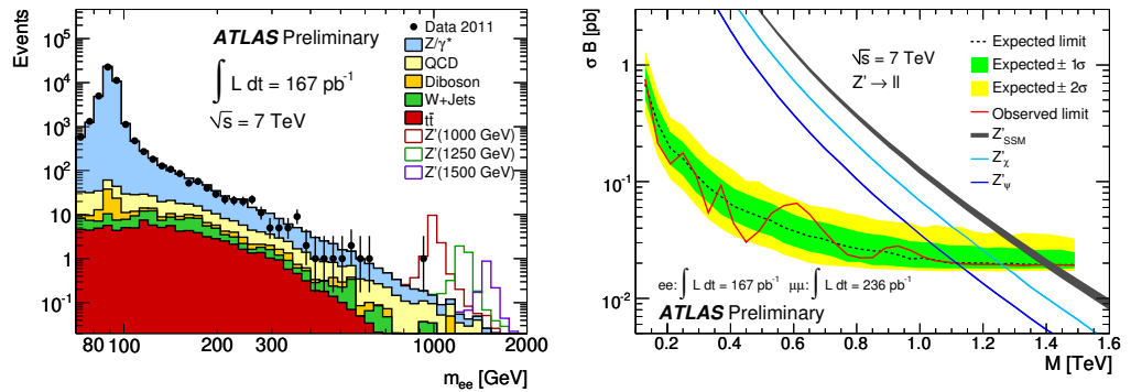
Figure 2: Invariant mass for dielectron events passing the Z' analysis selection (left). The open histograms show the expected contributions from three Z'_{SSM} mass hypotheses. Limits on \sigma B as a function of M_{Z'} combining the electron and muon channels (right). The curves show theoretical cross sections for various models.
