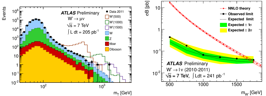
Figure 1: Transverse mass m_T for muon events passing the W' analysis selection (left). The open histograms show the expected contributions from three W'_{SSM} mass hypotheses. Limits on \sigma B as a function of M_{W'} combining the muon channel results described here with the electron channel results from 2010 (right). The red curve shows the theoretical cross-section, with errors, for the W'_{SSM} .
