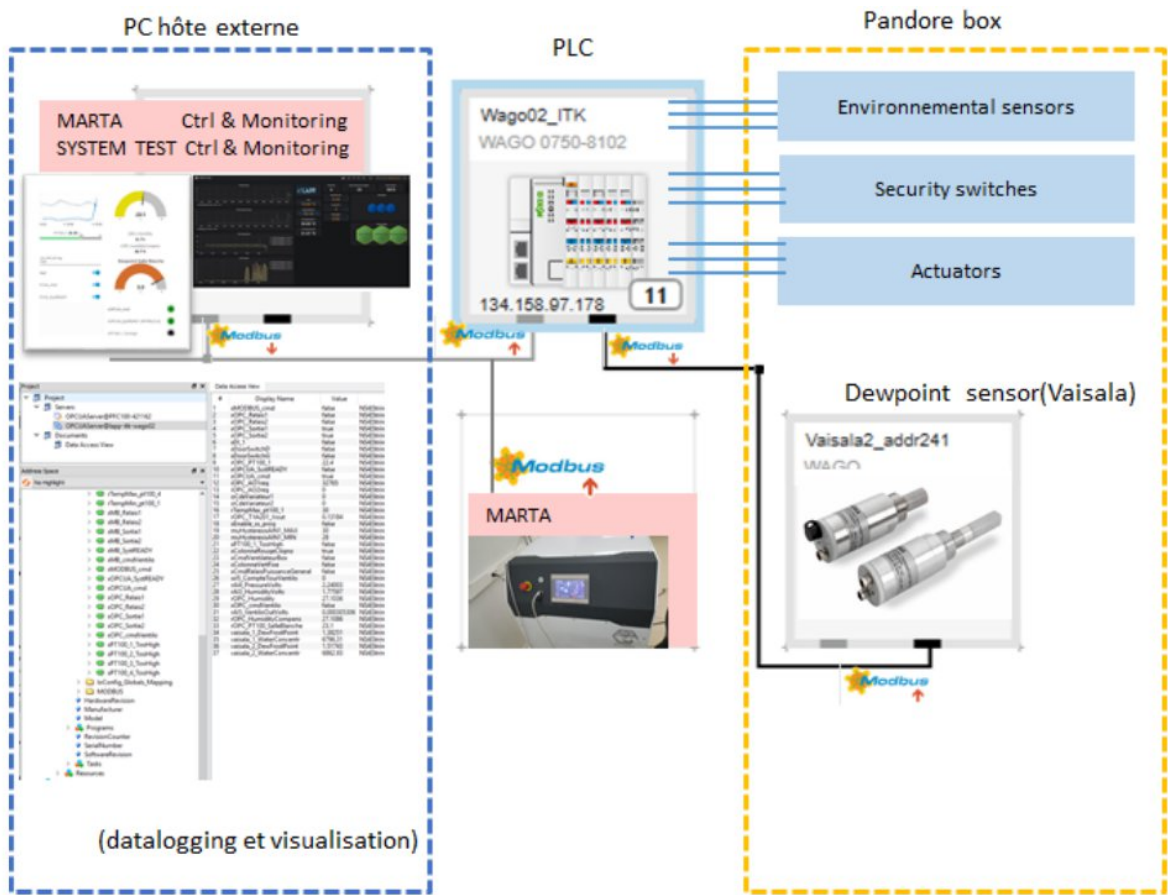
Figure 3. System test block diagram.
