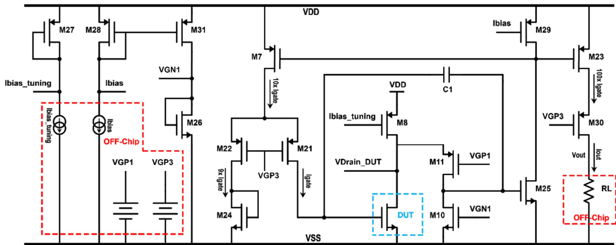
Fig. 1 - IGATE Amplifier transistor level schematic
