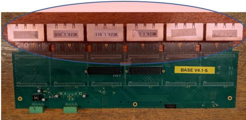
Figure 1: The BEC base board (green) and the 6 Mezzanines (red circle) – Front view.
