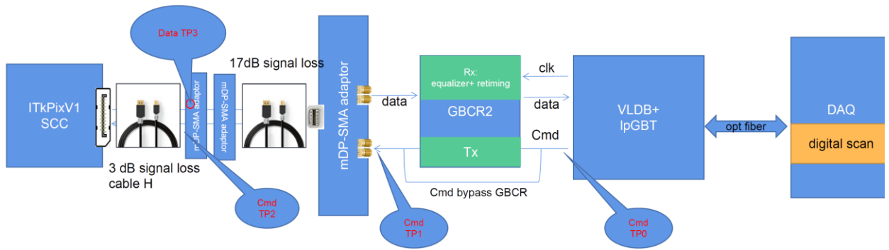
Figure 3: ATLAS ITk Pixel system data transmission demonstration
