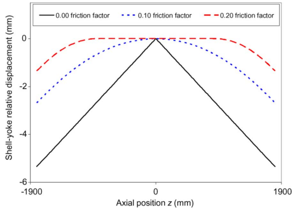
Fig. 5. Computed relative displacement (mm) between shell and yoke at 4.5 K with different friction factors, as a function of the shell axial position (mm).
