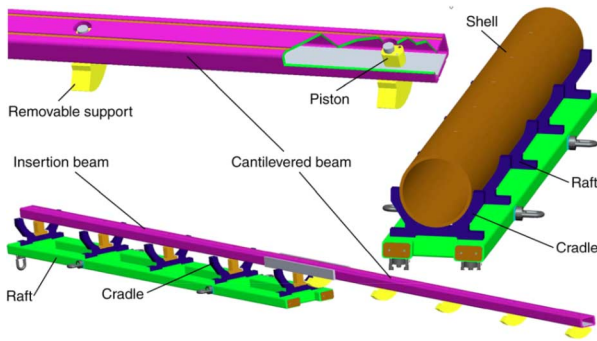
Fig. 3. Assembly tools: beams, cradles and rafts.
