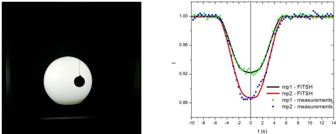
Fig. 1 Model star with transiting model planet [left]. Modelled (FITSH) and measured light curves obtained with two different size model planets (mp1 and mp2) [right].
