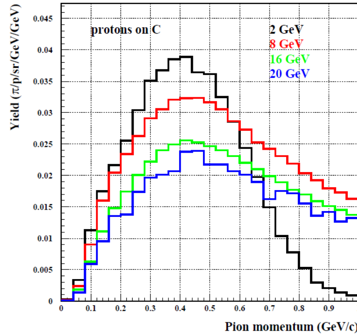
Carbon target
