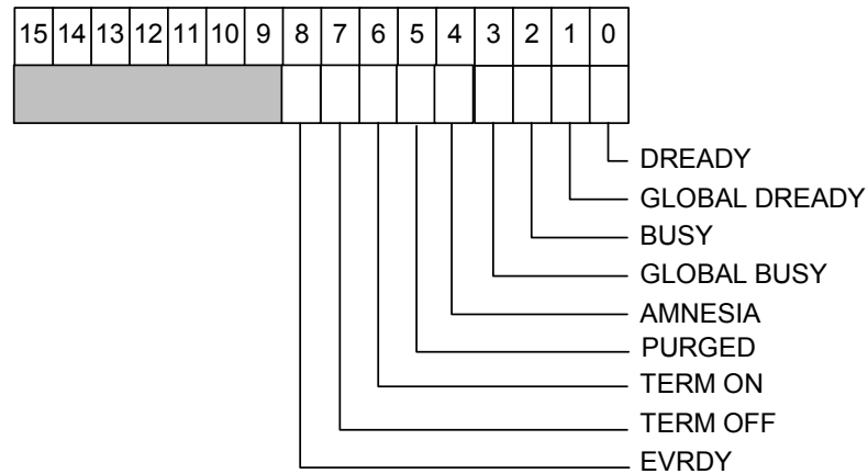
Fig. 4.16: Status Register 1
