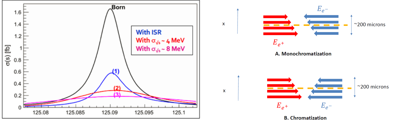
Fig. 1. Left: Higgs boson line shape. The e^+e^- \rightarrow H cross-section is shown as function of ECM. Black: at tree level; blue including initial state radiation; red (and magenta): adding the effect of a 4 (or 8) MeV ECM spread. Right: monochromatization. Top, the standard scheme with additional opposite sign horizontal dispersion in both beams. The average boost of the center-of-mass varies with the x-coordinate, so the knowledge of the ECM spread requires to make the measurement of the boost distribution as function of x. Bottom: a chromatization scheme in which ECM depends on the x-coordinate.
