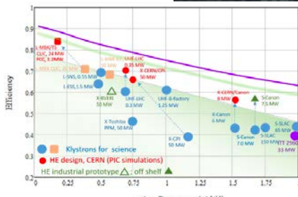
High-Efficiency Klystrons
