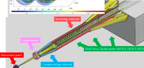
Magnets & SC magnets
