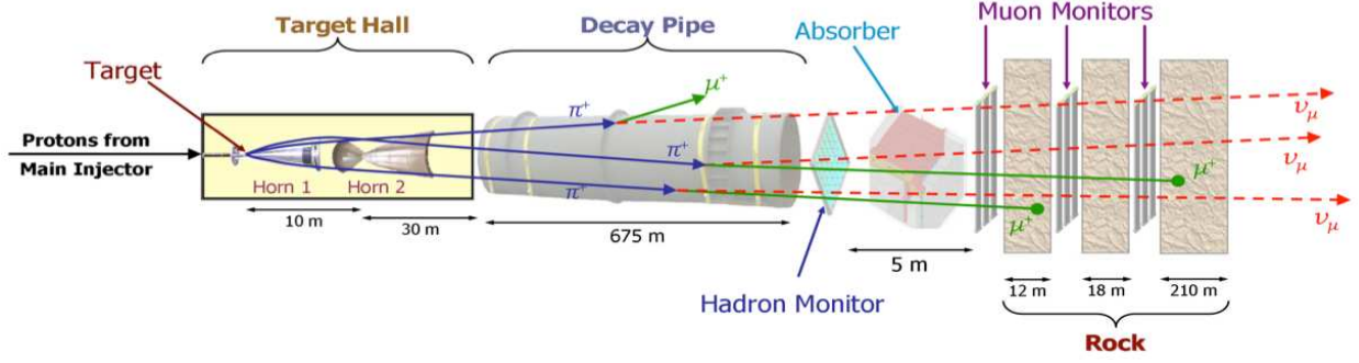
Figure 6: The NuMI beamline at Fermilab as described in [31].
