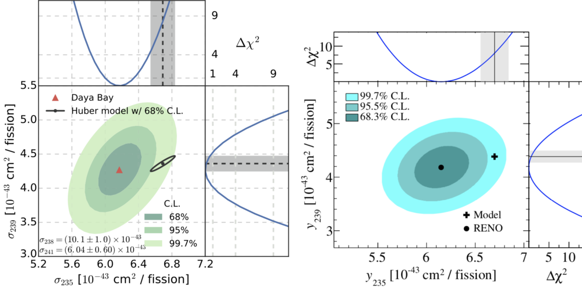
Figure 4: IBD yield per fission from ^{235}\text{U} vs. ^{239}\text{Pu} by Daya Bay (left) and RENO (right) from Refs. [15] and [16], respectively.
