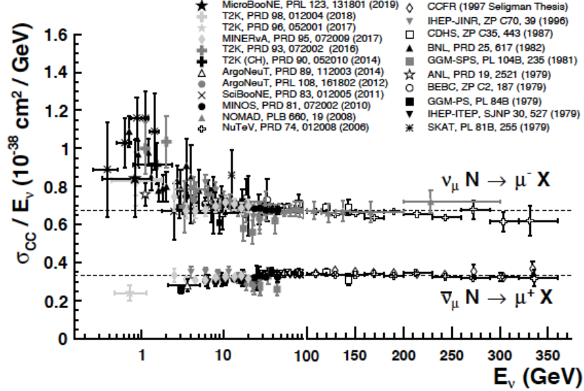
Figure 28: Neutrino inclusive cross sections scaled by neutrino energy from [277]. Quasi-elastic processes dominate at very low energies while partonic processes take over at higher energies.
