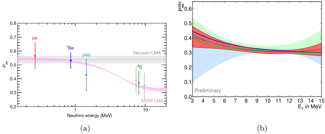
Figure 17: Electron neutrino survival probability P_{ee} as a function of their energy. (a) Data points represent the Borexino results, in which the error bars include experimental and theoretical uncertainties. The pink band is the \pm 1\sigma prediction of the MSW mechanism in matter, while the grey band is the case of vacuum-only oscillation. LMA label in the figure stands for the Large Mixing Angle, the current best-fit solution for solar oscillation parameters. From [48]. (b) Allowed survival probability 1\sigma band from the combined {}^8\text{B} solar neutrino data of Super-Kamiokande and SNO (red). The pastel colored bands are the separate Super-Kamiokande (green) and SNO (blue) fits. The solid lines are the MSW predictions using particular oscillation parameters resulting from the fit: to all solar data (green), all solar + KamLAND data (blue), to Super-Kamiokande and SNO data (robin egg blue). From [50].
