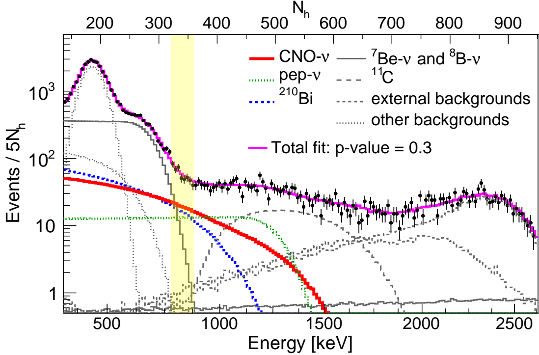
Figure 11: Spectral fit of the Borexino Phase-III data that lead to the observation of solar neutrinos from the CNO cycle shown in red. From [56].
