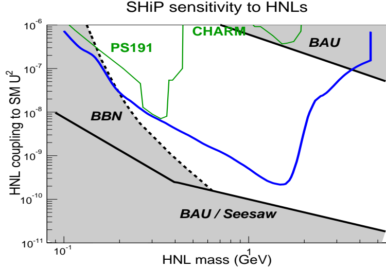
Figure 45: The white region displays mass and mixing of sterile neutrinos, here called HNL (Heavy Neutral Lepton), which can lead to successful resonant leptogenesis. Green lines are constraints from past experiments, the blue line is the expected sensitivity of SHiP. Taken from [596].
