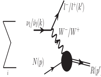
Figure 33: Diagrammatic representation of resonance excitations for the charged current induced \nu_\ell(\bar{\nu}_\ell) + N \rightarrow \ell^-(\ell^+) + R process, where R represents the different resonances contributing to the hadronic current.
