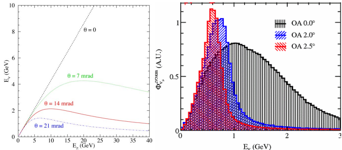
Figure 8: Dependence of neutrino energy on pion energy and angle relative to the secondary beam axis for the NuMI beamline [34] (left). Energy spectra for the off-axis T2K [35] beamline (right). The on-axis spectrum is shown, along with the optimized off-axis distribution.
