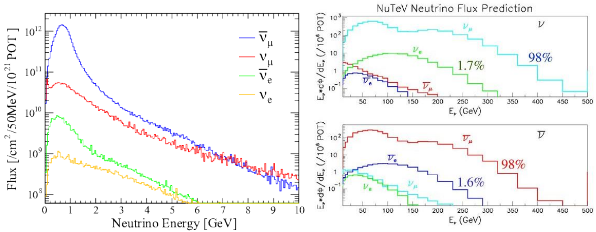
Figure 7: Composition of the low energy T2K [32] (left) and high energy (800 GeV protons) TeV II neutrino beam [33] at Fermilab (right, the relative contribution to the flux is indicated).
