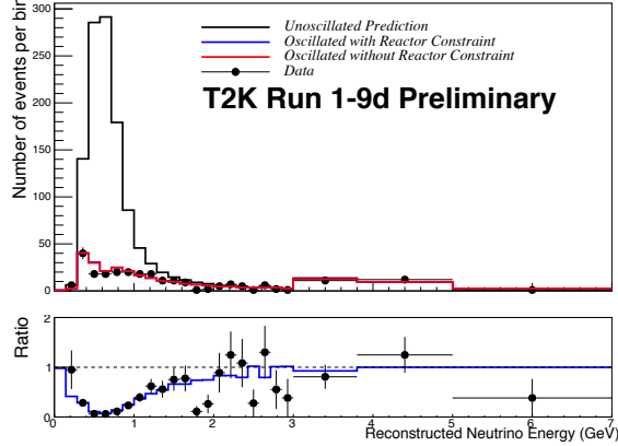
Figure 20: Neutrino energy spectrum measured using the Super-K detector (top). The data (solid points) are compared to the expected distribution in the absence of oscillations (black histogram) and the distribution that results when the best-fit values for \theta_{23} and \Delta m_{32}^2 are used. The ratio of the measured spectrum to the unoscillated spectrum is shown in the lower panel. The blue line shows the expectations of the best-fit spectrum.
