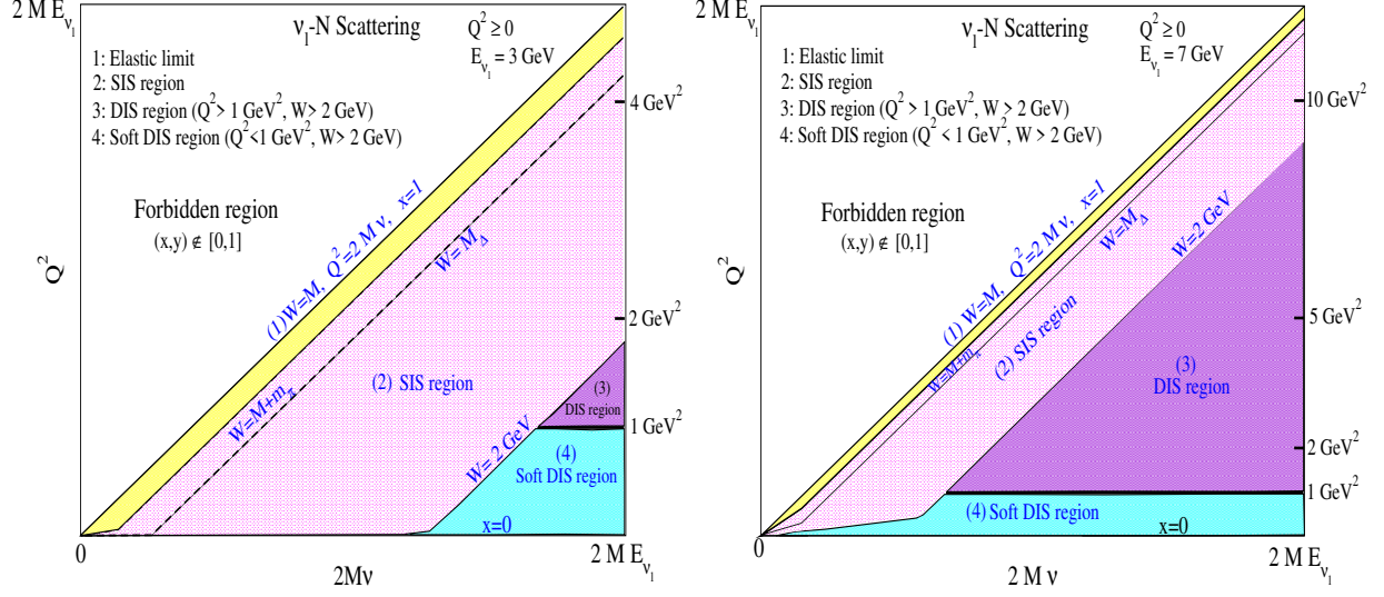
Figure 31: Allowed kinematical region for neutrino-nucleon scattering in the (Q^2, \nu) plane for E_\nu = 3 \text{ GeV} (left panel) and E_\nu = 7 \text{ GeV} (right panel). The square of the invariant mass is defined as W^2 = M_N^2 + 2M_N\nu - Q^2 with nucleon mass M_N and energy transfer \nu . The inelasticity is defined as y = \frac{\nu}{E_\nu} = \frac{(E_\nu - E_l)}{E_\nu} and the forbidden region in terms of x and y is then defined as x, y \notin [0, 1] . The elastic limit is x = \frac{Q^2}{2M_N\nu} = 1 and the shallow inelastic scattering (SIS) region is defined as the region for which M_N + M_\pi \leq W \leq 2 \text{ GeV} and Q^2 \geq 0 covering both non-resonant and resonant meson production. The DIS region is defined as the region for which Q^2 \geq 1 \text{ GeV}^2 and W \geq 2 \text{ GeV} , and the soft DIS region is defined as Q^2 < 1 \text{ GeV}^2 and W \geq 2 \text{ GeV} . Notice the yellow band ( M_N < W < M_N + M_\pi ), where we do not expect anything from neutrino-nucleon scattering. However, this region becomes important when the scattering takes place with a nucleon within a nucleus due to the multi-nucleon correlation effect. In the yellow band process like photon emission is possible. Soft DIS region is also nothing but the SIS region. The boundaries between regions are not sharply established and are indicative only.
