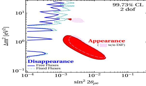
Figure 41: Appearance versus disappearance data for the relevant mixing parameters \sin^2 2\theta_{e\mu} = 4|U_{e4}U_{\mu4}| and \Delta m_{41}^2 at 99.73% C.L. for 2 dof. Disappearance data using free reactor fluxes (solid) or fixed reactor fluxes (dashed) are used. The allowed parameters are to the left of the dark and light blue lines. The shaded contours in red (pink hatched) are the allowed parameters from appearance data including (excluding) decay-in-flight LSND results. Taken from Ref. [587].
