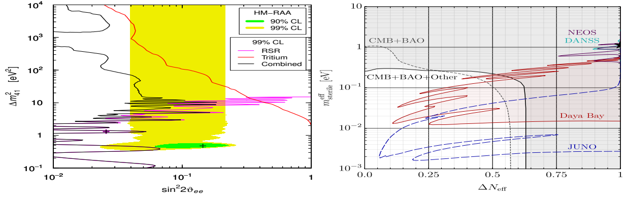
Figure 43: The left plot shows in green and yellow the 90% and 99% C.L. areas coming from the reactor flux deficit solution, while the pink line shows the result of an analysis of reactor experiments with spectral ratio measurements (RSR). A combination of Mainz, Troitsk and KATRIN tritium experiments is seen in red, which can be combined with the RSR fit to the black line. Taken from Ref. [574]. Here \sin^2 2\theta_{ee} = 4|U_{e4}|^2(1 - |U_{e4}|^2) . The right plot shows constraints in the plane of \Delta N_{\text{eff}} and sterile neutrino mass from reactor experiments, including prospects of the future JUNO project. Taken from [591].
