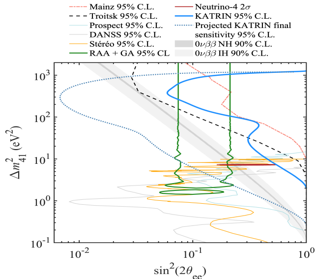
Figure 40: KATRIN’s 95% C.L. constraints on sterile neutrino parameters in comparison with fits to the reactor and gallium anomalies, as well as with dedicated reactor neutrino experiments looking for sterile neutrinos. A comparison to neutrinoless double beta decay is also made. Taken from Ref. [317].
