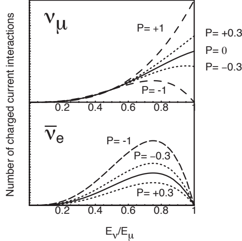
Figure 9: Neutrino spectra from a 20 GeV muon storage ring. For a given muon polarization, P , the muon and electron neutrino spectra are fixed by the beam energy.
