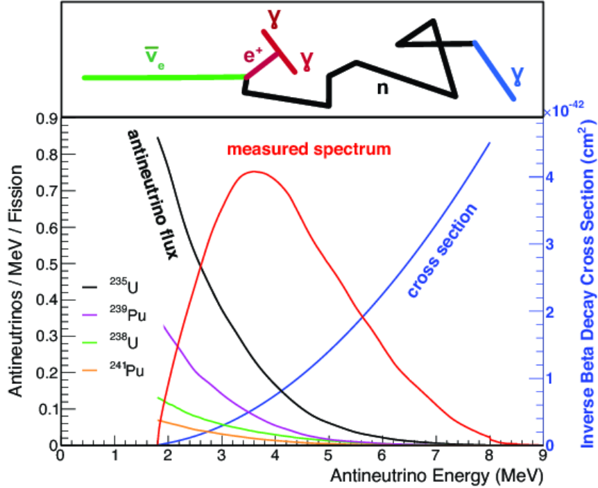
Figure 2: Reactor neutrino fluxes for the four main isotopes (black, violet, green and orange), IBD cross section (blue) and corresponding measurable neutrino spectrum (red).
