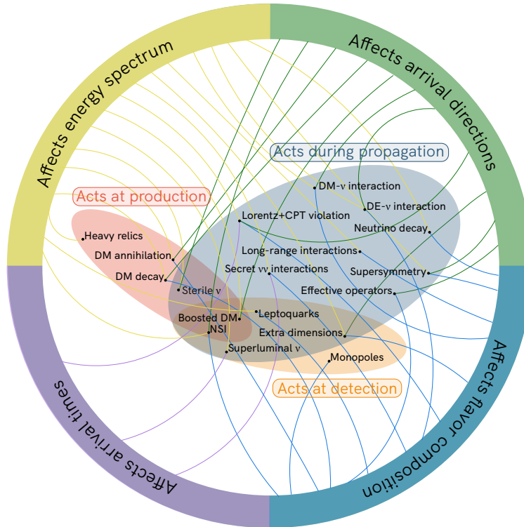
Figure 48: Possible mechanisms for BSM physics testable with astrophysical neutrinos. Figure taken from [696].
