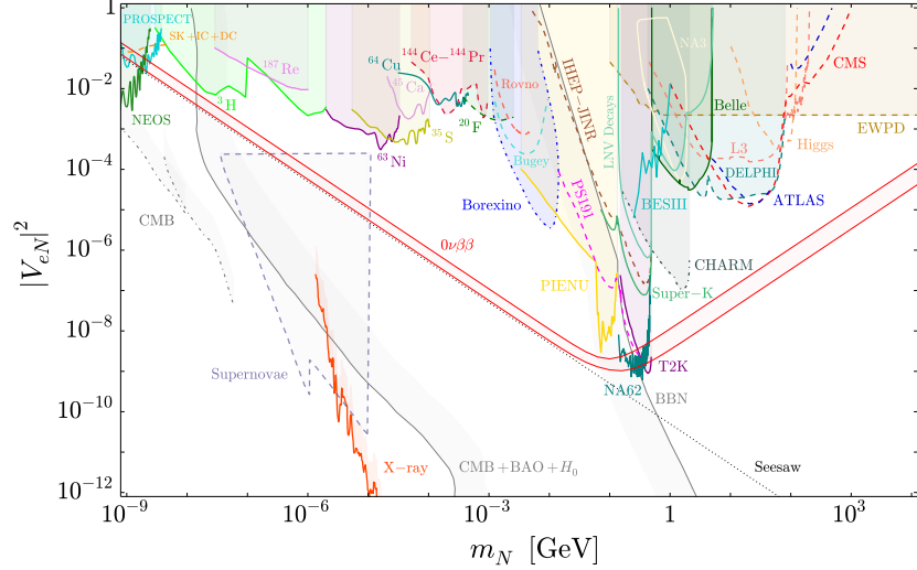
Figure 44: Constraints on the mass of a sterile neutrino and its mixing with electron neutrinos from a variety of astroparticle and particle physics searches. Taken from [595].
