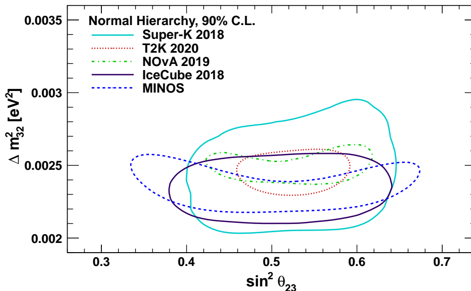
Figure 15: Neutrino mixing parameter measurements from both atmospheric (Super-Kamiokande [245] and IceCube [244]) and accelerator (T2K [246], NOvA [247], and MINOS [31]) neutrino experiments.
