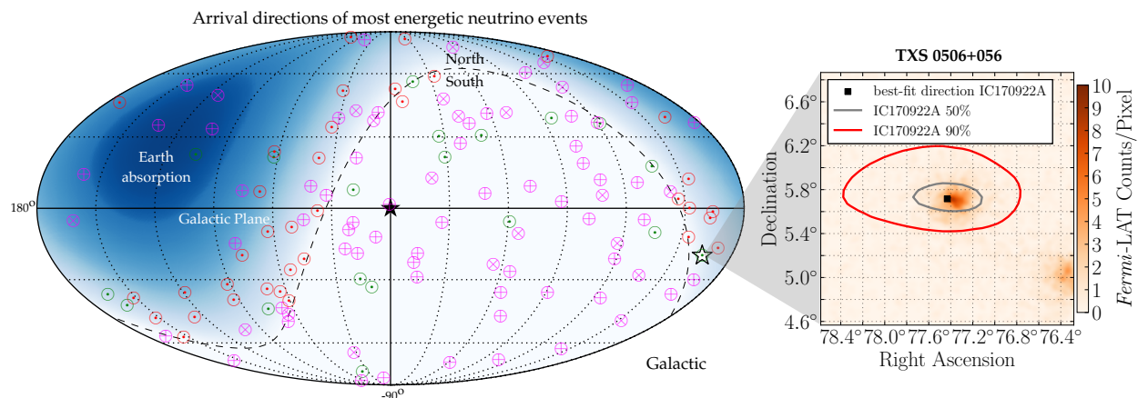
Figure 14: The current sky map of highly energetic neutrino events detected by IceCube. Shown are upgoing track events [129, 186], the high-energy starting events (HESE) and cascades [160, 187, 188], and additional track events published as public alerts [189]. The distribution of the events is largely isotropic. The location of the first compelling neutrino source, blazar TXS 0506+056, is marked with a star. Shown in the inset are the related Fermi Large Area Telescope (LAT) measurements of the region centred on TXS 0506+056 from September 2017 [147]. The uncertainty ellipses of the IceCube neutrino event IC-170922A are shown for reference.
