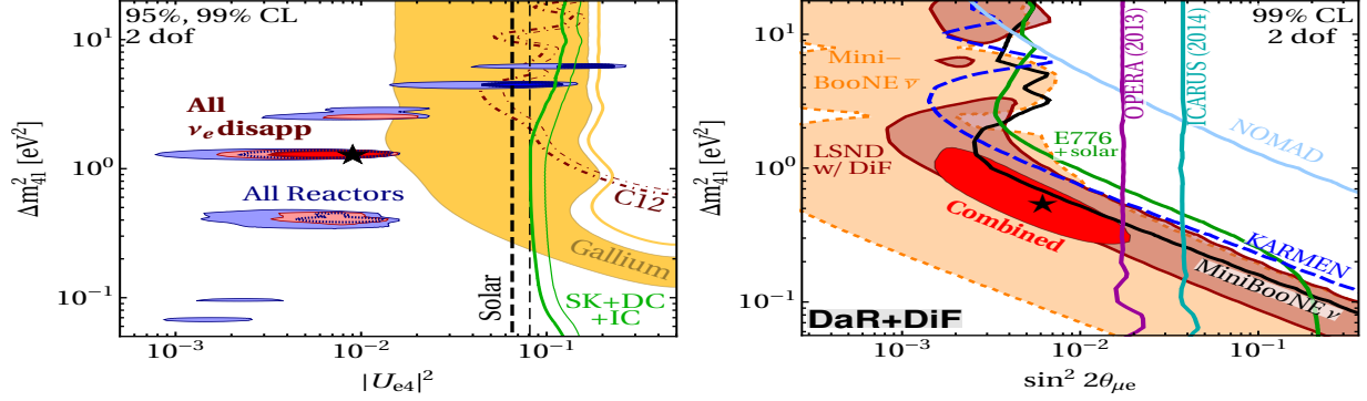
Figure 42: Fit results on sterile neutrinos using only \nu_e \rightarrow \nu_e disappearance (left) and \nu_\mu \rightarrow \nu_e appearance (right). Taken from Ref. [587].
