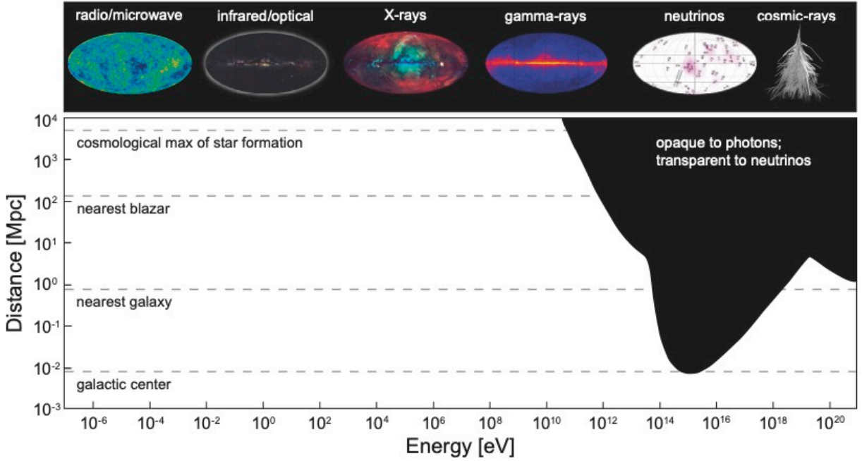
Figure 13: Distance horizon at which the Universe becomes intransparent to electromagnetic radiation [138].
