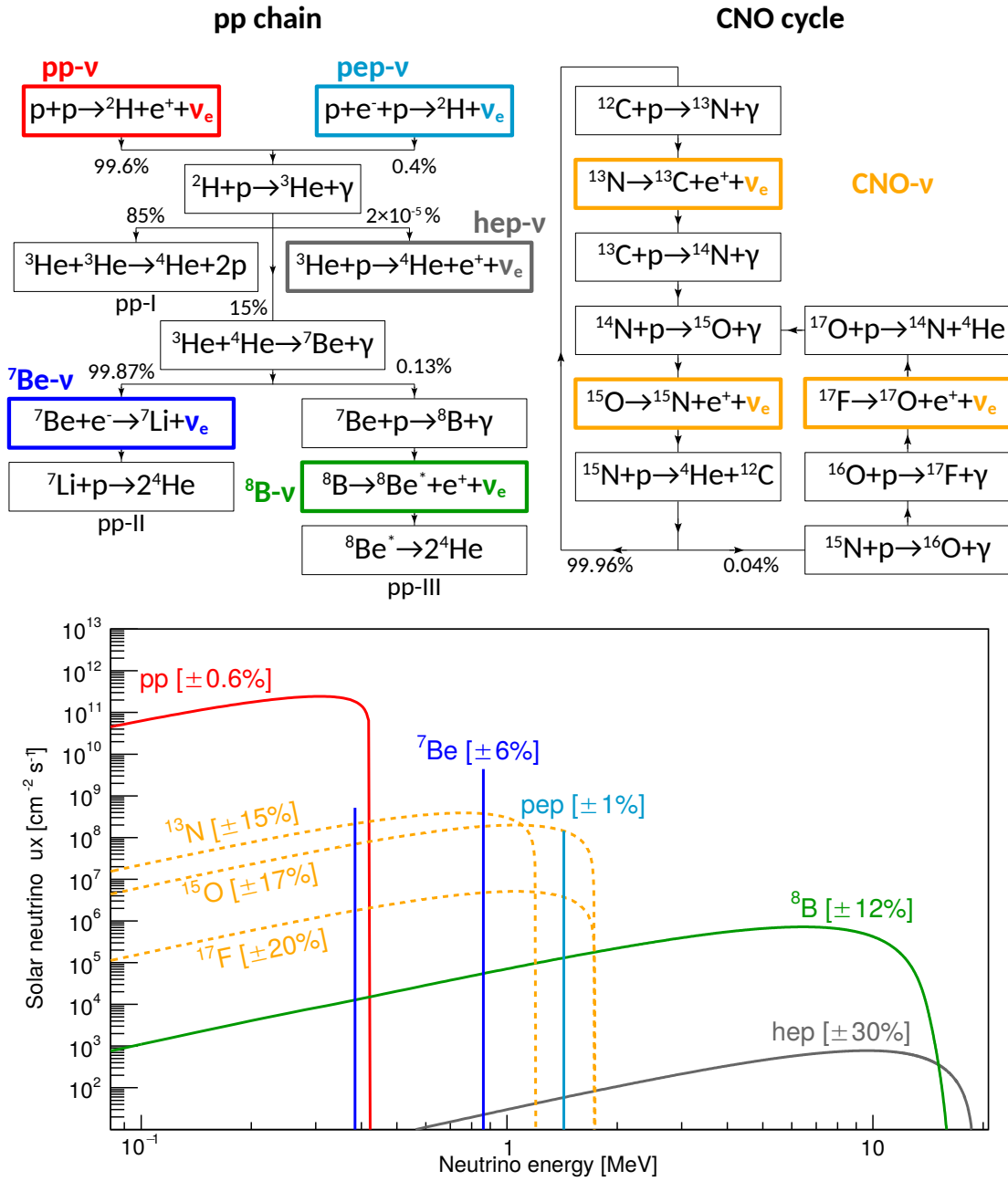
Figure 10: Top: Nuclear fusion sequences occurring in the core of the Sun: schematic view of the pp -chain and the CNO cycle. Bottom: Solar neutrino energy spectrum with fluxes from [57]. The flux (vertical scale) is given in \text{cm}^{-2} \text{s}^{-1} \text{MeV}^{-1} for continuous sources and in \text{cm}^{-2} \text{s}^{-1} for mono-energetic ones. From [48].
