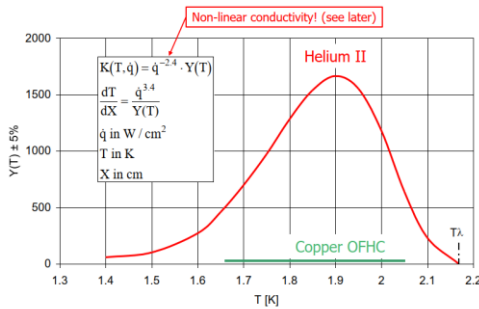
Equivalent thermal conductivity of He II p
