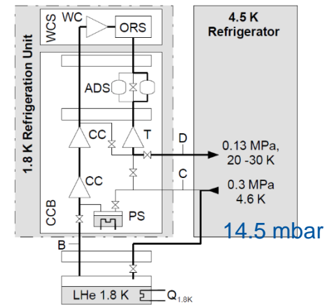
2.4 kW 1.8 K refrigeration unit
