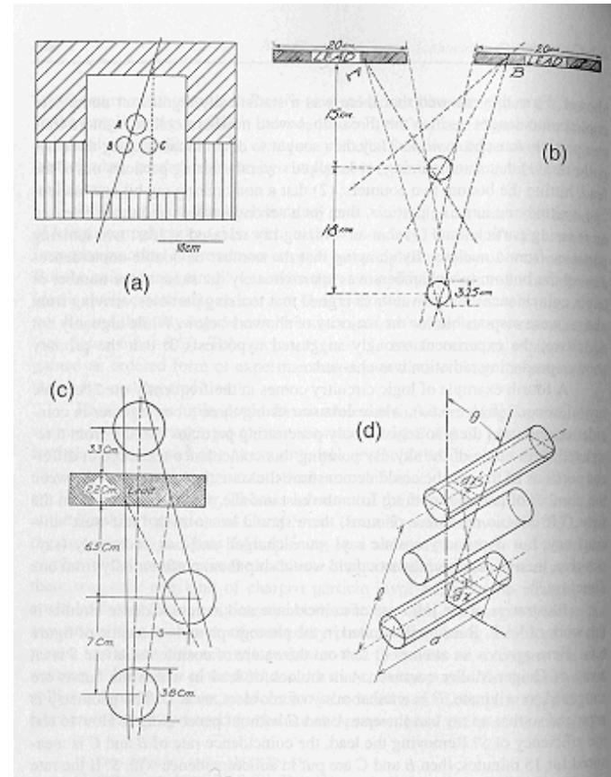
Early coincidence counting experiment
