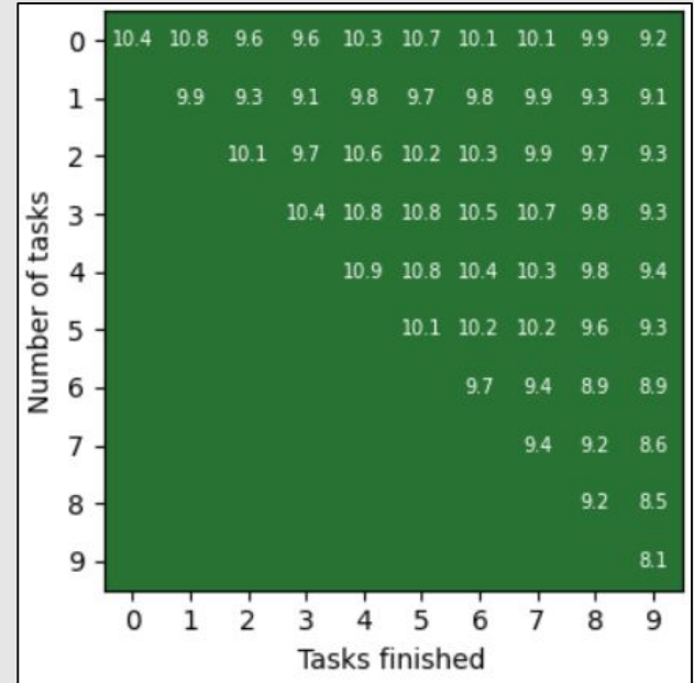
Wasserstein distance on all channels with continuously increased amount of data
