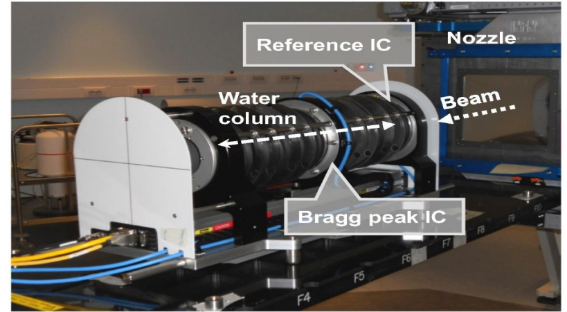
PTW Peakfinder system (IC – Ionization Chamber)
