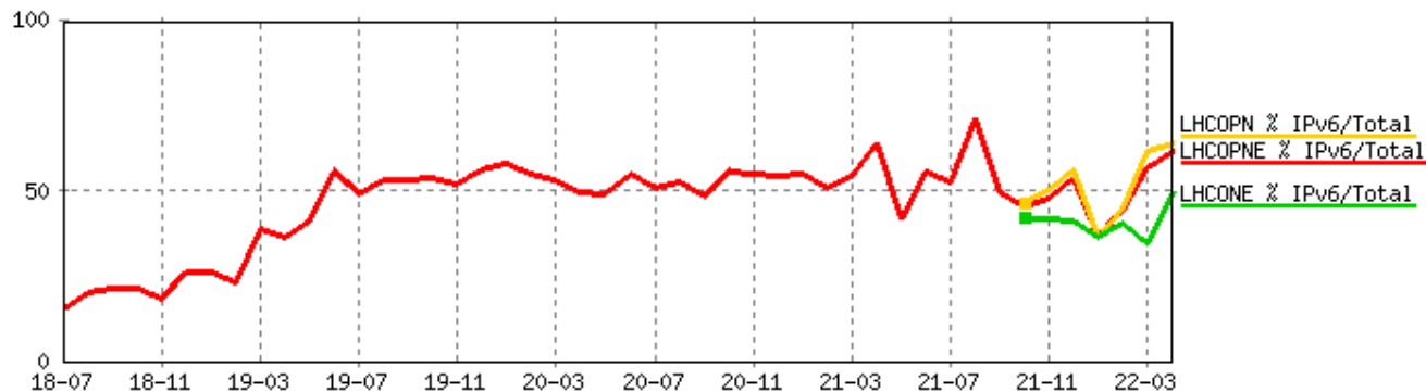
Percentage of IPv6 traffic over the total
