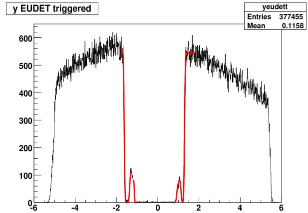
Fig.4: Vertical tomography of upper and lower detector edges with small peaks indicating the windows.
