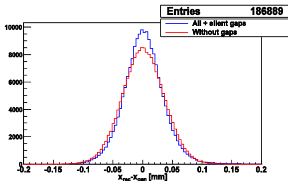
Fig.3 Typical resolution of an ALFA fibre detector.
