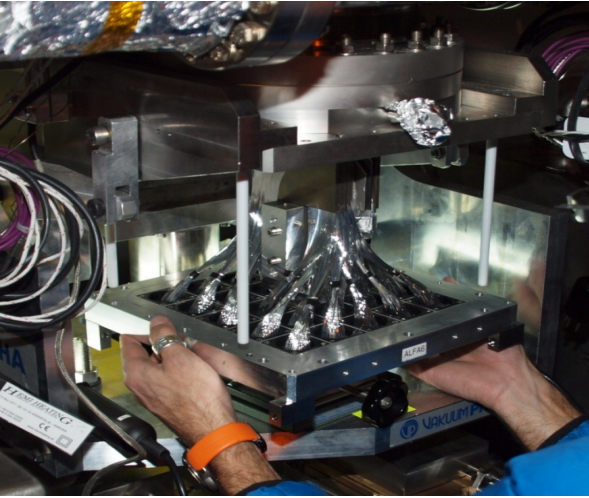
Fig.5: Insertion of a lower fibre detector in the RomanPot.
