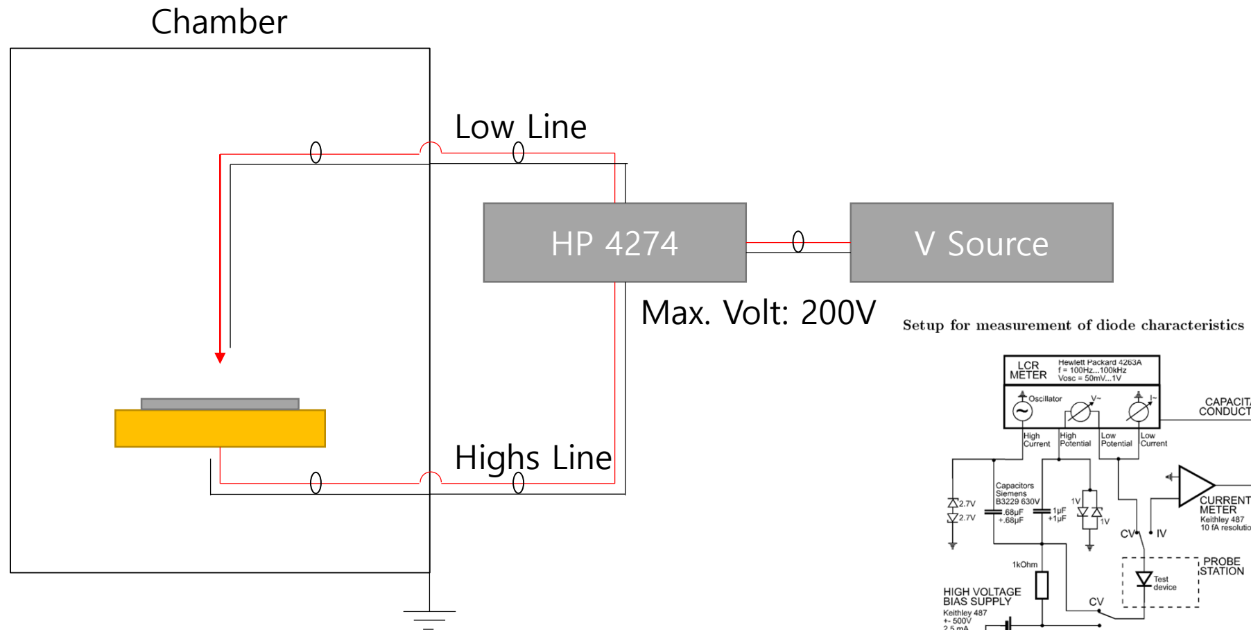
Figure 4.5: Electrical setup for C/V and I/V measurements (taken from [Fei97a]).
