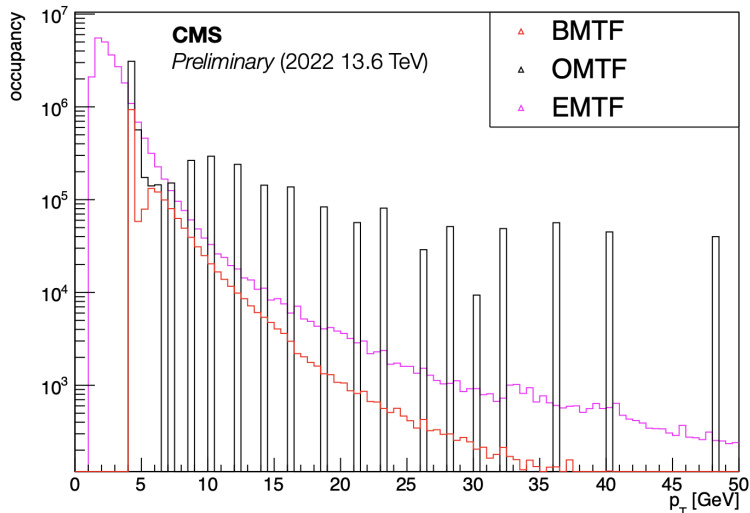
Figure 1. The p_T distribution of L1 muons, from the BMTF(red), OMTF(black), and EMTF(pink). Data captured by the L1DS demonstrator from 100k orbits (about 9 seconds of data taking) in 2022 with 2448 colliding bunches at 6.8 TeV beam energy. The coarse binning for the OMTF values is a result of the quantisation in the FPGA logic for estimating the p_T . [5]
