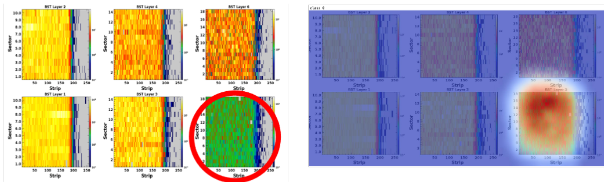
Figure 5. Left: A typical online monitoring histogram from Hall B. The red circle indicates a low occupancy, as identified by the detector expert. Right: The original image with a GradCAM heat map overlaid, identifying the regions of the image that are important for the specific classification.
