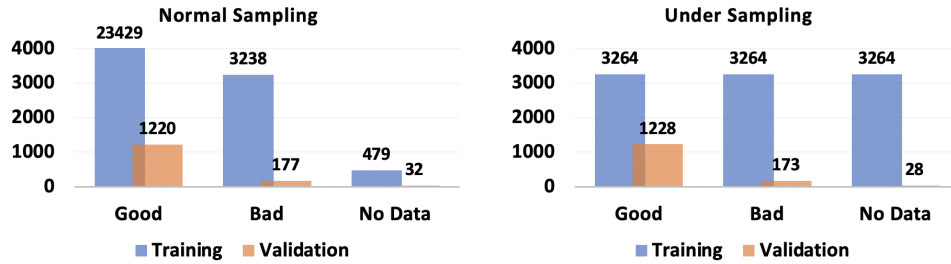
Figure 2. 'Normal' and 'Under' sampling schemes. Note the counts are different between the two schemes due to changes in random selection. Given enough statistics the 'Under' sampling scheme produces models just as accurate as other sampling methods in around one-fifth the time.
