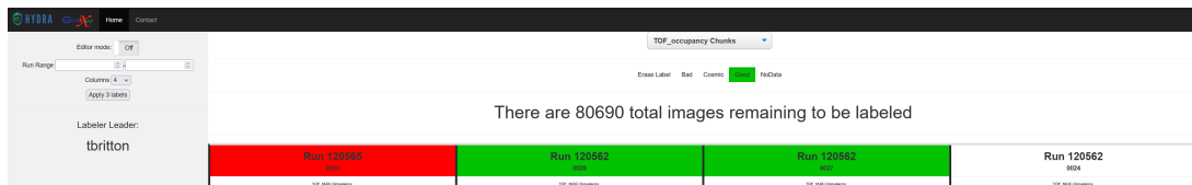
Figure 1. The Data Labeler web page. Monitoring histograms are sorted by detector and run number. Each image can then be quickly labeled utilizing the available labels that appear above the set of images. The images and labels are stored in a database to be used for training.
