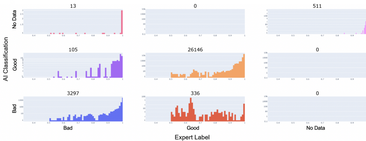
Figure 3. An example 'enhanced' confusion matrix. In this matrix all combinations of AI prediction and Expert Labels are plotted; the number above the distribution represents the count in each element and when taken alone is the standard confusion matrix. The distribution represents the confidence (between 0.0 and 1.0) the model had in its classification.
