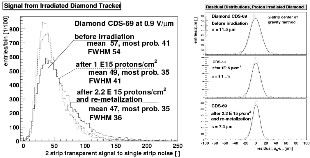
Figure 21: (a) Transparent 2-strip charge signal-to-noise distributions before (solid line), after proton irradiations with 1 \times 10^{15} p/cm 2 (dashed line) and after 2.2 \times 10^{15} p/cm 2 (dotted line). (b) Residual distributions before and after proton irradiation.
