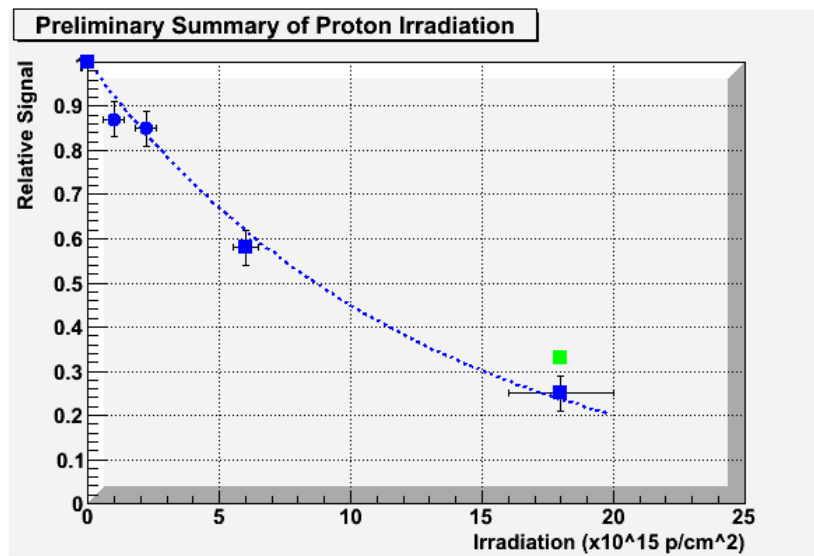
Figure 22: Summary of proton irradiation results for pCVD material at an electric field of 1 V/μm (solid circle points) and 2 V/μm (solid square point) to a fluence of 18 \times 10^{15} p/cm 2 . The blue curve is an exponential with exponent -0.08 \times \text{fluence} to guide the eye.
