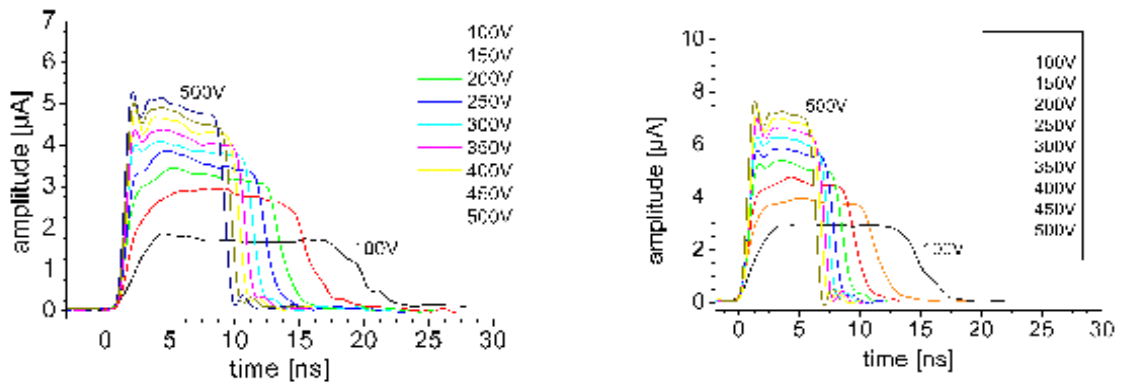
Figure 6: The observed current pulses created by alpha particles injected on one surface of the scCVD diamond as a function of time.
