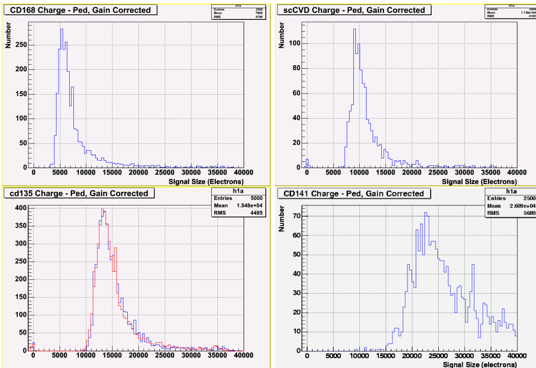
Figure 4: The pulse height distribution of various scCVD diamonds. The thicknesses of the diamonds are, from top left to to bottom right 210, 330, 435, 685 \mu\text{m} . When there are two curves they are the results for positive and negative applied voltage.
