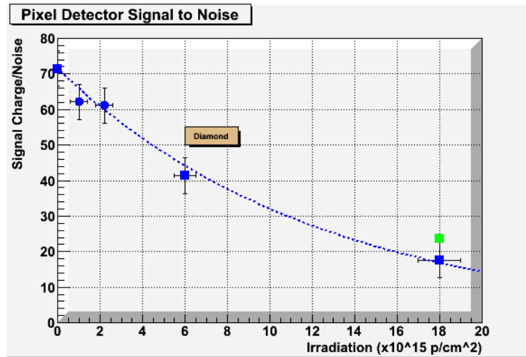
Figure 24: The expected Signal-to-Noise for irradiated diamond pixel modules.
