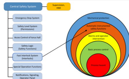
Fig. 3: Fast Interlock System as a part of the safety system for W7-X machine protection
