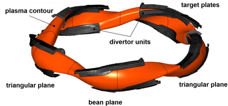
Fig. 2: Actively cooled divertor units
