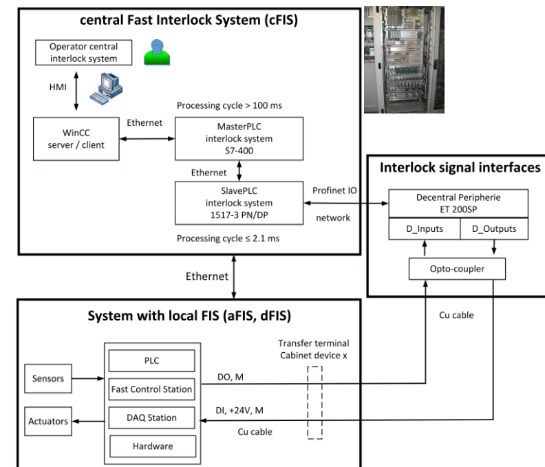
Fig. 3: Structure of FIS
