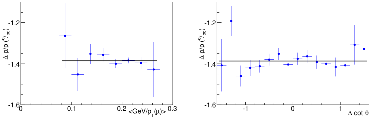
FIG. S11: Fractional momentum shift \Delta p/p (per mille) from \Upsilon \rightarrow \mu\mu data as a function of \langle 1/p_T^\mu \rangle (left) and \Delta \cot \theta (right). The measurements include corrections to the ionization energy loss determined from J/\psi \rightarrow \mu\mu decays that remove \langle 1/p_T^\mu \rangle dependence, and to the COT scale and twist determined from \Upsilon \rightarrow \mu\mu decays that remove \Delta \cot \theta dependence. Fits to a constant are overlaid on the plots as a visual aid.
