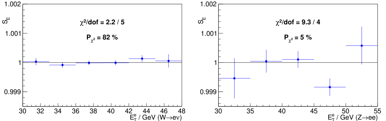
FIG. S15: Measured energy scale as a function of electron E_T for W \rightarrow e\nu (left) and Z \rightarrow ee (right) data, with the line S_E = 1 overlaid. The simulation is corrected with the best-fit value of \zeta = (7.2 \pm 0.4) \times 10^{-3} in Eq. (S1).
