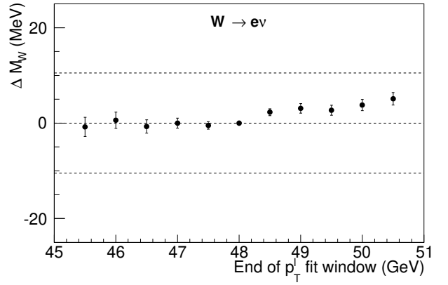
FIG. S40: Variations of the M_W value determined from the charged-lepton transverse-momentum fit as a function of the choice of the lower (top) and upper (bottom) edge of the fit range, for the muon (left) and electron (right) channels. Uncertainty bars indicate the expected statistical variation with respect to the default fit range, as computed using pseudoexperiments. The dashed lines indicate the statistical uncertainty from the default mass fit.
