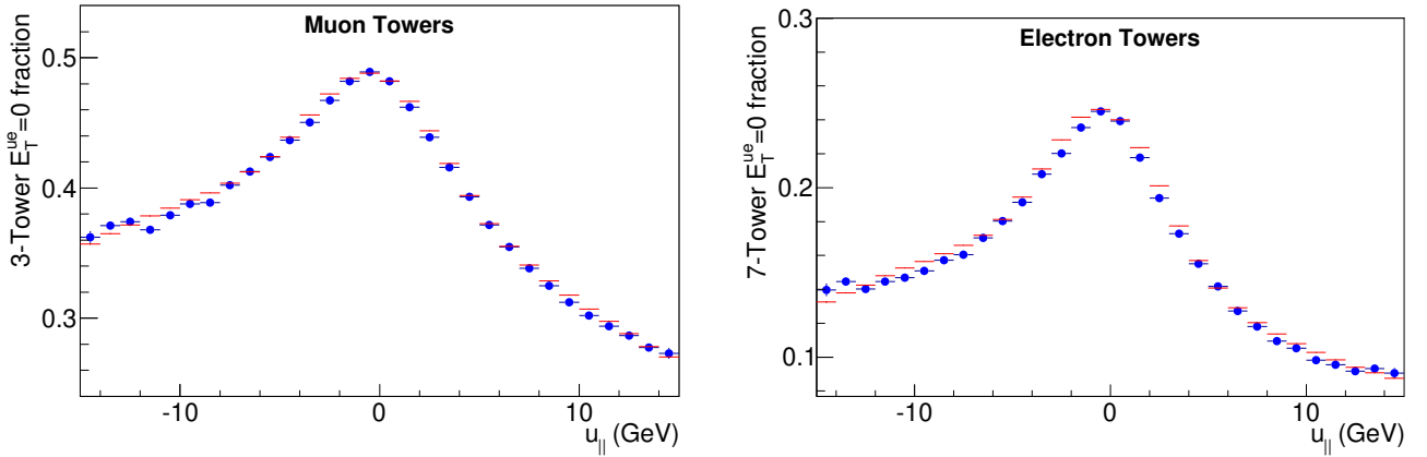
FIG. S19: Fraction of muon-data three-tower (left) and electron-data seven-tower (right) rotated windows containing zero energy, as a function of u_{||} . The red lines show the simulation, while the blue circles show the data.
