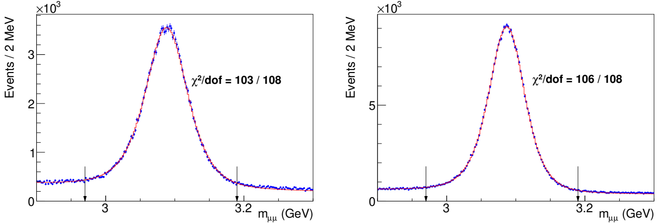
FIG. S9: Representative dimuon mass fits (histogram) to data (circles), in the ranges \langle 1/p_T^\mu \rangle = (0.15, 0.1625) \text{GeV}^{-1} (left) and \langle 1/p_T^\mu \rangle = (0.1875, 0.2) \text{GeV}^{-1} (right) of the J/\psi \rightarrow \mu\mu data. The arrows enclose the fit range. Each fitting template includes a linear background shape which is separately constrained by including wider sidebands in the fit region.
