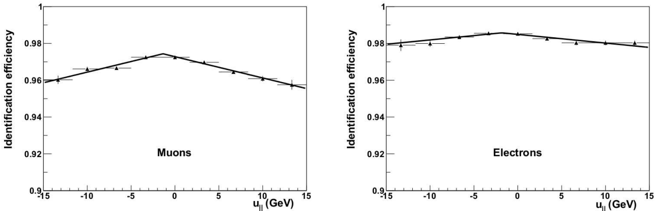
FIG. S4: Muon (left) and electron (right) identification efficiency as a function of the recoil component in the direction of the lepton ( u_{\parallel} ), as measured in Z \rightarrow \ell\ell data using the tag-probe technique. The piece-wise linear fits are used to model the lepton efficiencies in the simulation.
