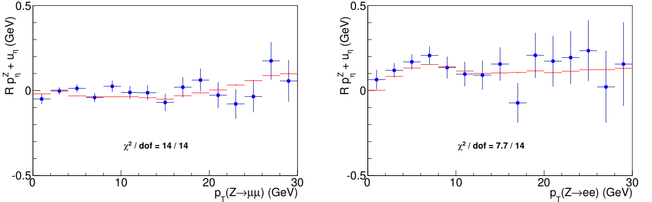
FIG. S23: Distribution of R p_{\eta}^{\ell\ell} + u_{\eta} for Z -boson decays to muons (left) and electrons (right) as a function of Z -boson p_T in simulated (lines) and experimental (circles) data. The detector response parameters a and b (Eq. S15) are obtained by minimizing the combined \chi^2 of these distributions.
