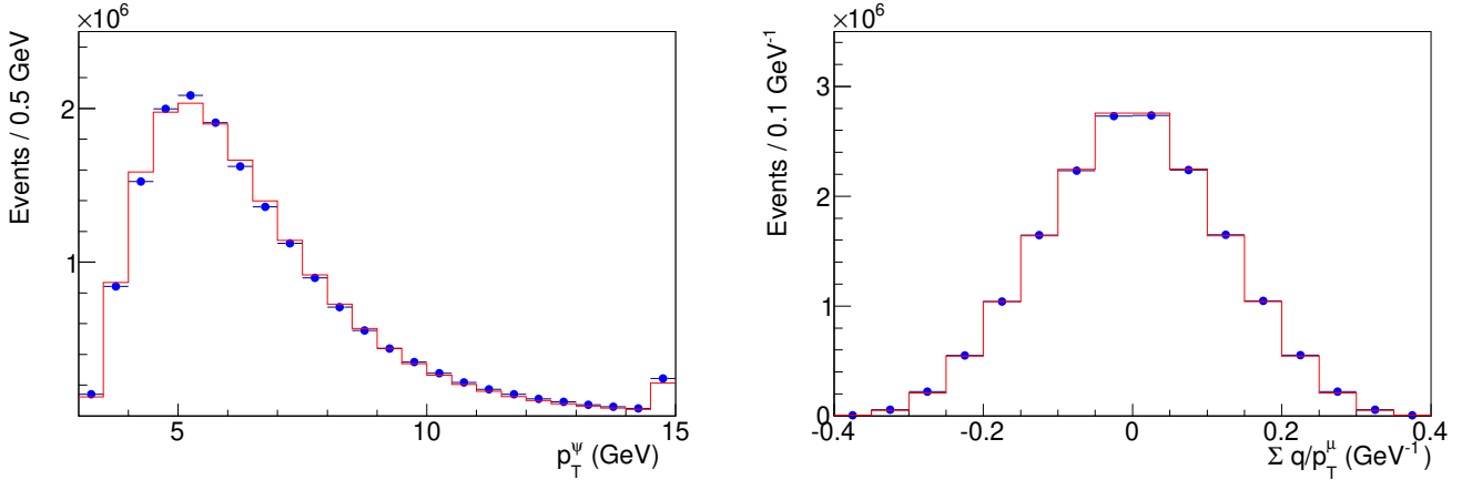
FIG. S7: Distribution of dimuon p_T (left) and \Sigma(q/p_T^\mu) (right) in the data (circles) and the simulation of J/\psi \rightarrow \mu\mu decays (histogram). The data distributions are background-subtracted using events in the mass range 3.17–3.31 GeV.
