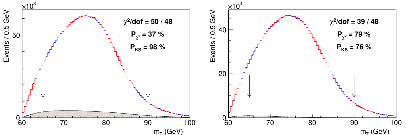
FIG. S33: Distributions of m_T for W boson decays to \mu\nu (left) and e\nu (right) final states in simulated (histogram) and experimental (points) data. The simulated distribution is based on the true W -boson mass value that maximizes the likelihood in data and includes backgrounds (shaded). The likelihood is computed using events between the two arrows.
