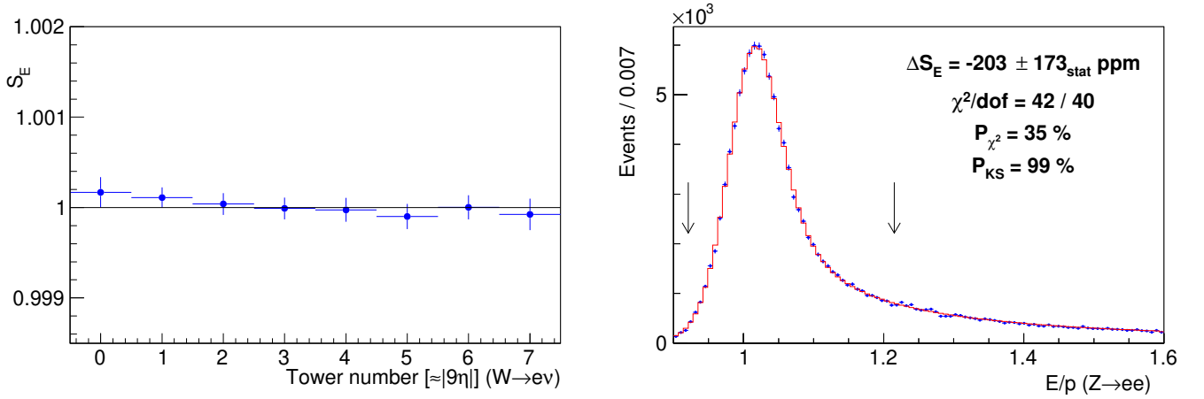
FIG. S13: (Left) Measured calorimeter energy scale in bins of electron tower in W \rightarrow e\nu data after corrections are applied, with the line S_E = 1 overlaid. The towers are numbered in order of increasing |\eta| and each tower subtends \Delta\eta \approx 0.11 . (Right) Distribution of E/p for Z \rightarrow ee data (circles) after the full energy-scale calibration; the best-fit template (histogram) is overlaid. The fit region is enclosed by arrows.
