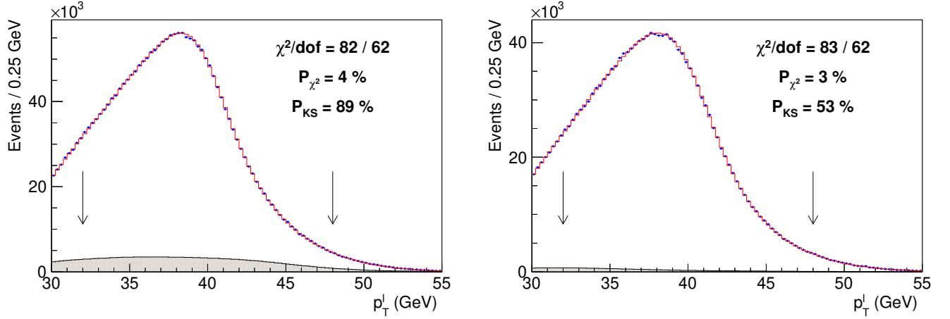
FIG. S34: Distributions of p_T^l for W boson decays to \mu\nu (left) and e\nu (right) final states in simulated (histogram) and experimental (points) data. The simulated distribution is based on the true W -boson mass value that maximizes the likelihood in data and includes backgrounds (shaded). The likelihood is computed using events between the two arrows.
