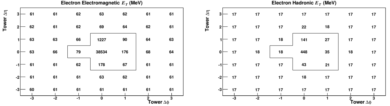
FIG. S18: Average measured energy (in MeV) in the electromagnetic (left) and hadronic (right) calorimeters in the vicinity of the electron shower in W -boson decays. The differences \Delta\phi and \Delta\eta are signed such that positive differences correspond to towers closest to the electron shower position at the CEM. The seven towers inside the box are removed from the recoil measurement.
