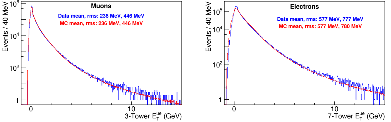
FIG. S21: Distribution of hadronic E_T in the three-tower (left) and seven-tower (right) window separated in azimuth by 90^\circ from the muon or electron, respectively. The red histogram shows the hadronic E_T modeled in the custom simulation, while the blue histogram shows the data. The negative values occur due to the luminosity-dependent correction.
