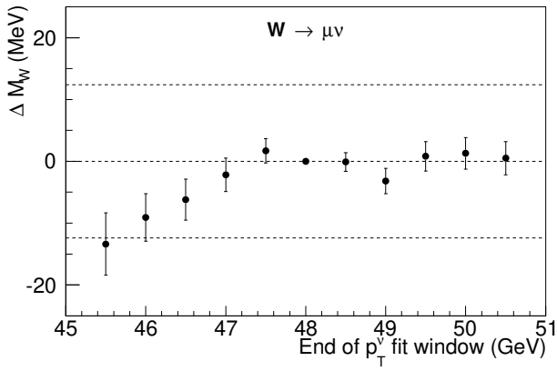
FIG. S41: Variations of the M_W value determined from the neutrino-transverse-momentum fit as a function of the choice of the lower (top) and upper (bottom) edge of the fit range, for the muon (left) and electron (right) channels. Uncertainty bars indicate the expected statistical variation with respect to the default fit range, as computed using pseudoexperiments. The dashed lines indicate the statistical uncertainty from the default mass fit.
