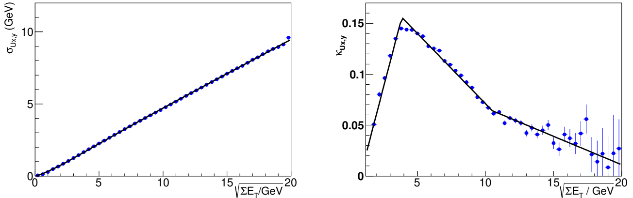
FIG. S30: (left) rms of u_x and u_y in minimum-bias data, shown as a function of the scalar \sqrt{\Sigma E_T} . The black curve is the function given by Eq. (S26). (right) Excess kurtosis \kappa of the distribution of (u_i - \langle u_i \rangle)/\sigma_i ( i = x, y ) in minimum-bias data, shown as a function of the scalar \sqrt{\Sigma E_T} . The black curve is a piece-wise linear fit used in the custom detector simulation.
