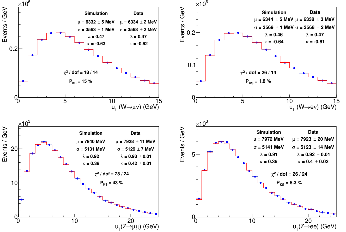
FIG. S32: Distributions of u_T from simulation (histogram) and data (circles) for W boson (top) and Z boson (bottom) decays in the muon (left) and electron (right) channels. The simulation uses parameters fit from Z boson data, and the uncertainty on the simulation is due to the statistical uncertainty on these parameters. The data mean ( \mu ), rms spread ( \sigma ), skewness ( \lambda ), and excess kurtosis ( \kappa ) are well modeled by the simulation. The \chi^2 values and the Kolmogorov-Smirnov (KS) probabilities are based only upon the statistical uncertainties in the data and do not take into account the systematic uncertainties in the simulation.
