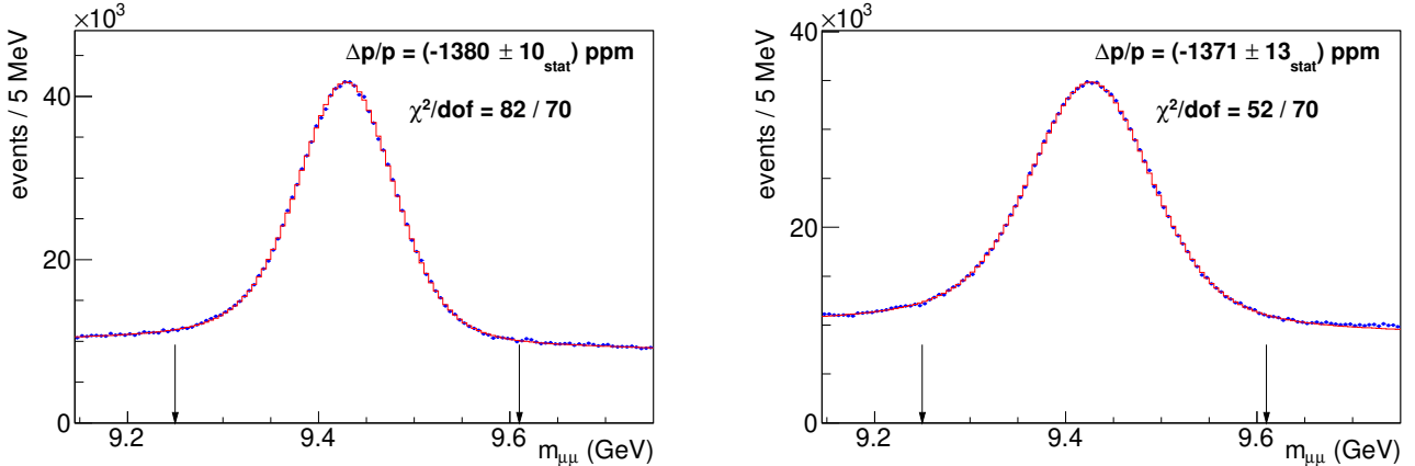
FIG. S12: Distribution of dimuon mass for the best-fit templates (histograms) and the data (circles) in the \Upsilon \rightarrow \mu\mu sample used to calibrate the muon momentum scale. The muon tracks are reconstructed with (left) or without (right) a constraint to the beam position in the transverse plane. The arrows enclose the fit range. Each fitting template includes a background shape which is separately constrained by including wider sidebands in the fit region.
