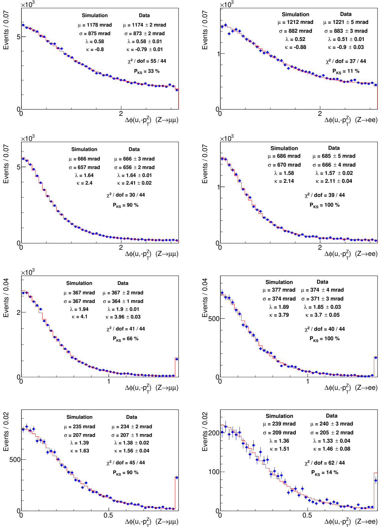
FIG. S26: Distributions of the difference in azimuthal angles of \vec{u} and -\vec{p}_T^{\ell\ell} , shown in absolute value in the following p_T^{\ell\ell} ranges: (top) p_T^{\ell\ell} < 8 GeV, (2nd row) 8 < p_T^{\ell\ell} < 15 GeV, (3rd row) 15 < p_T^{\ell\ell} < 23 GeV and (bottom) 23 < p_T^{\ell\ell} < 30 GeV. The distributions from Z \rightarrow \mu\mu events are shown on the left and those from Z \rightarrow ee events are shown on the right. The data (blue circles) are compared to the tuned simulation (red histogram).
