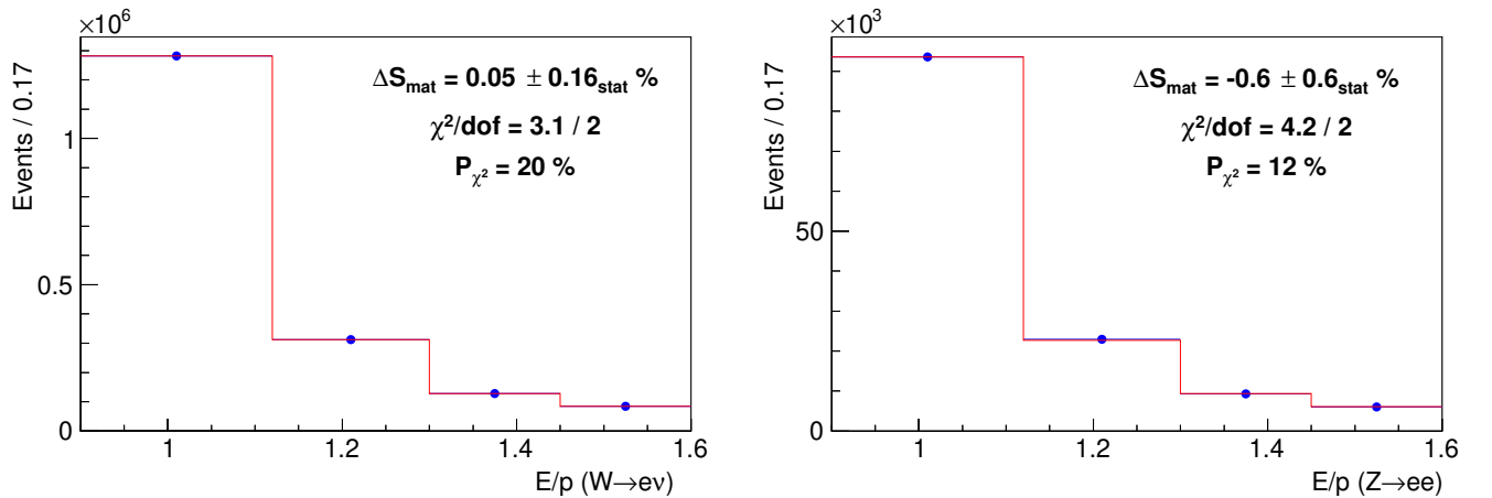
FIG. S14: Distributions of E/p in data (circles) and simulation with the best-fit value of S_{\text{mat}}^{W,Z} (histograms) in W \rightarrow e\nu (left) and Z \rightarrow ee (right) events.
