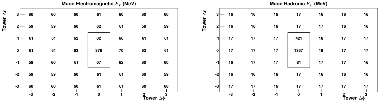
FIG. S17: Average measured energy (in MeV) in the electromagnetic (left) and hadronic (right) calorimeters in the vicinity of the muon in W -boson decays. The differences \Delta\phi and \Delta\eta are signed such that positive differences correspond to towers closest to the muon position at the CEM shower-maximum. The three towers inside the box are removed from the recoil measurement.
