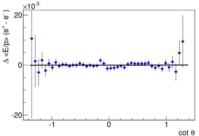
FIG. S6: Difference in \langle E/p \rangle between positrons and electrons as a function of \cot \theta , and its linear fit. The curvature corrections given in Eq. (S4) have been applied.
