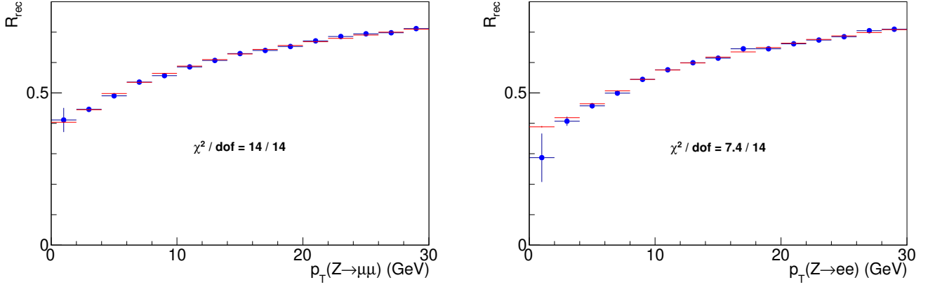
FIG. S22: Mean value of R_{\text{rec}} \equiv -\vec{u}_T \cdot \hat{p}_T^{\ell\ell} / p_T^{\ell\ell} , which approximates the recoil response R , as a function of dimuon p_T (left) and dielectron p_T (right). The distributions motivate the logarithmic parametrization of the response in Eq. (S15). The simulation (red lines) models the data (blue circles) accurately.
