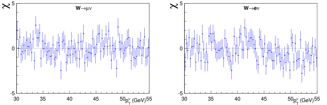
FIG. S38: Differences between the data and simulation, divided by the expected statistical uncertainty, for the p_T^\nu distributions in the muon (left) and electron (right) channels.
