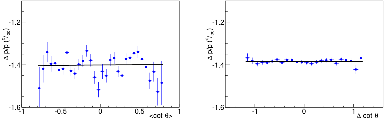
FIG. S8: (left) Measured \Delta p/p (per mille) as a function of the mean \cot \theta of the muon pair from J/\psi decay, after requiring |\Delta \cot \theta| < 0.1 and including corrections. (right) Measured \Delta p/p as a function of \Delta \cot \theta of the muon pair from J/\psi decay, after including corrections.
