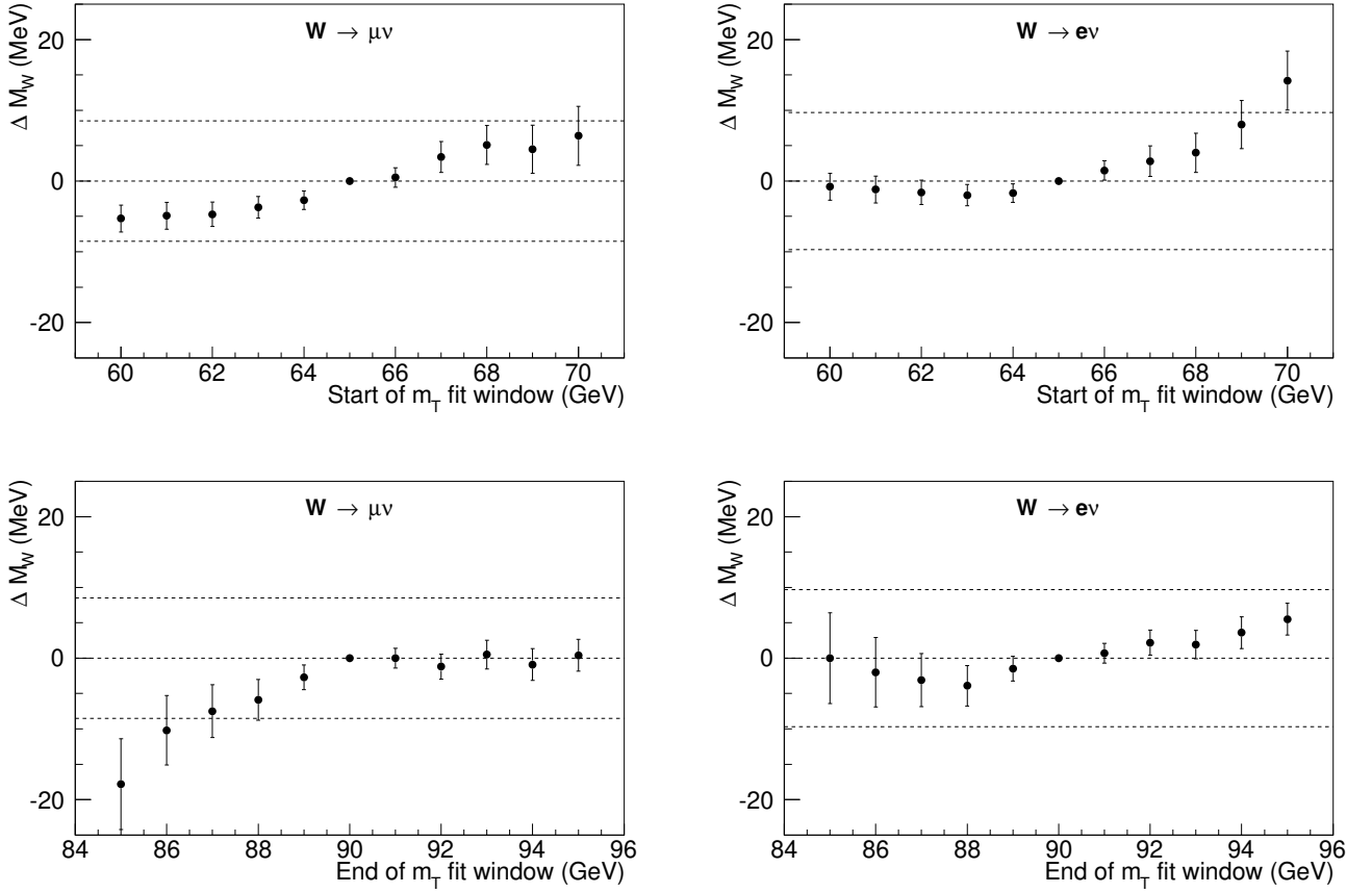
FIG. S39: Variations of the M_W value determined from the transverse-mass fit as a function of the choice of the lower (top) and upper (bottom) edge of the fit range, for the muon (left) and electron (right) channels. Uncertainty bars indicate the expected statistical variation with respect to the default fit range, as computed using pseudoexperiments. The dashed lines indicate the statistical uncertainty from the default mass fit.
