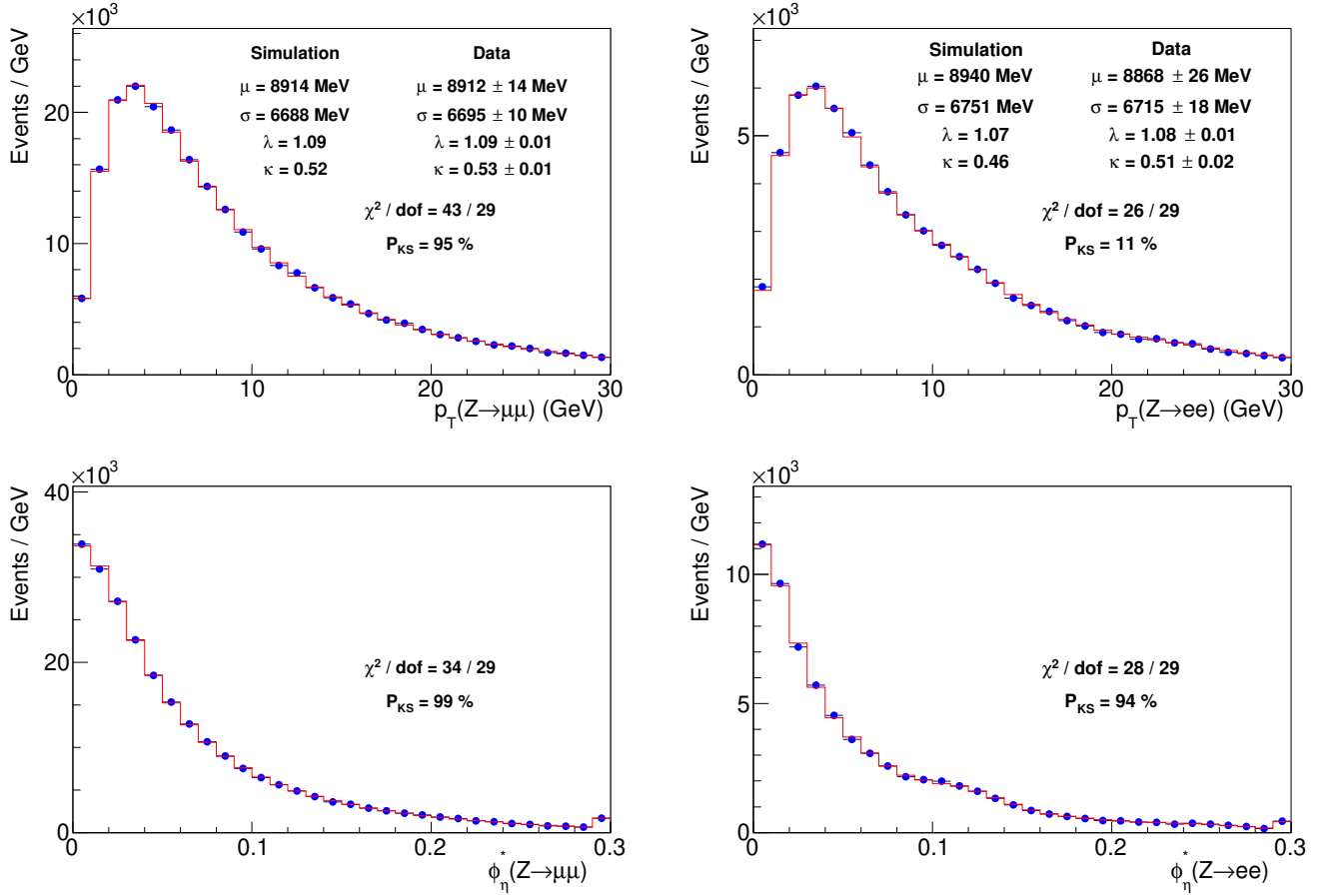
FIG. S2: Distributions of p_T^Z (top) and \phi_\eta^* (bottom) from simulation (histogram) and data (circles) for Z -boson decays to \mu\mu (left), and to ee (right). The p_T^Z distributions are used to fit for the nonperturbative parameter g_2 and for \alpha_s , and the \phi_\eta^* distributions provide a consistency check. The \phi_\eta^* distribution in the electron channel is modulated by the periodic azimuthal acceptance of the 24 calorimeter wedges. In these and other figures, “ P_{KS} ” refers to the Kolmogorov-Smirnov probability of agreement between the shapes of the data and simulated distributions.
