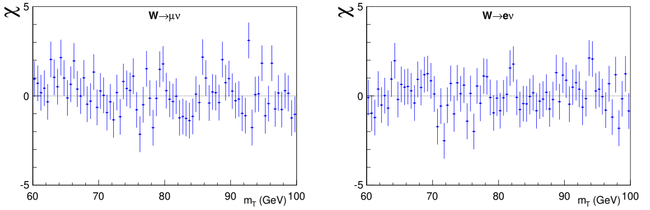
FIG. S36: Differences between the data and simulation, divided by the expected statistical uncertainty, for the m_T distributions in the muon (left) and electron (right) channels.
