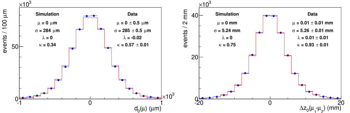
FIG. S1: Comparisons of the distributions of the impact parameter d_0 (left) and the difference of z_0 values (right) for the muon tracks in Z \rightarrow \mu\mu data (circles) and simulation (histogram). The cumulants of the distributions, rms ( \sigma ), skewness ( \lambda ) and excess kurtosis ( \kappa ) are in adequate agreement.
