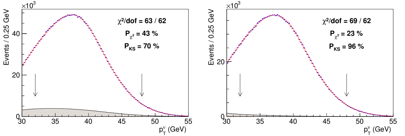
FIG. S35: Distributions of p_T^\nu for W boson decays to \mu\nu (left) and e\nu (right) final states in simulated (histogram) and experimental (points) data. The simulated distribution is based on the true W -boson mass value that maximizes the likelihood in data and includes backgrounds (shaded). The likelihood is computed using events between the two arrows.
