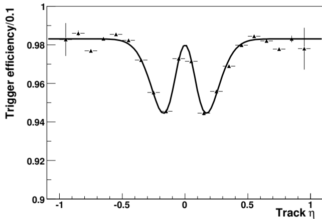
FIG. S5: Track trigger efficiency as a function of track \eta for electrons identified in the calorimeter. The measurement used W -boson events collected with a trigger with no track requirement.
