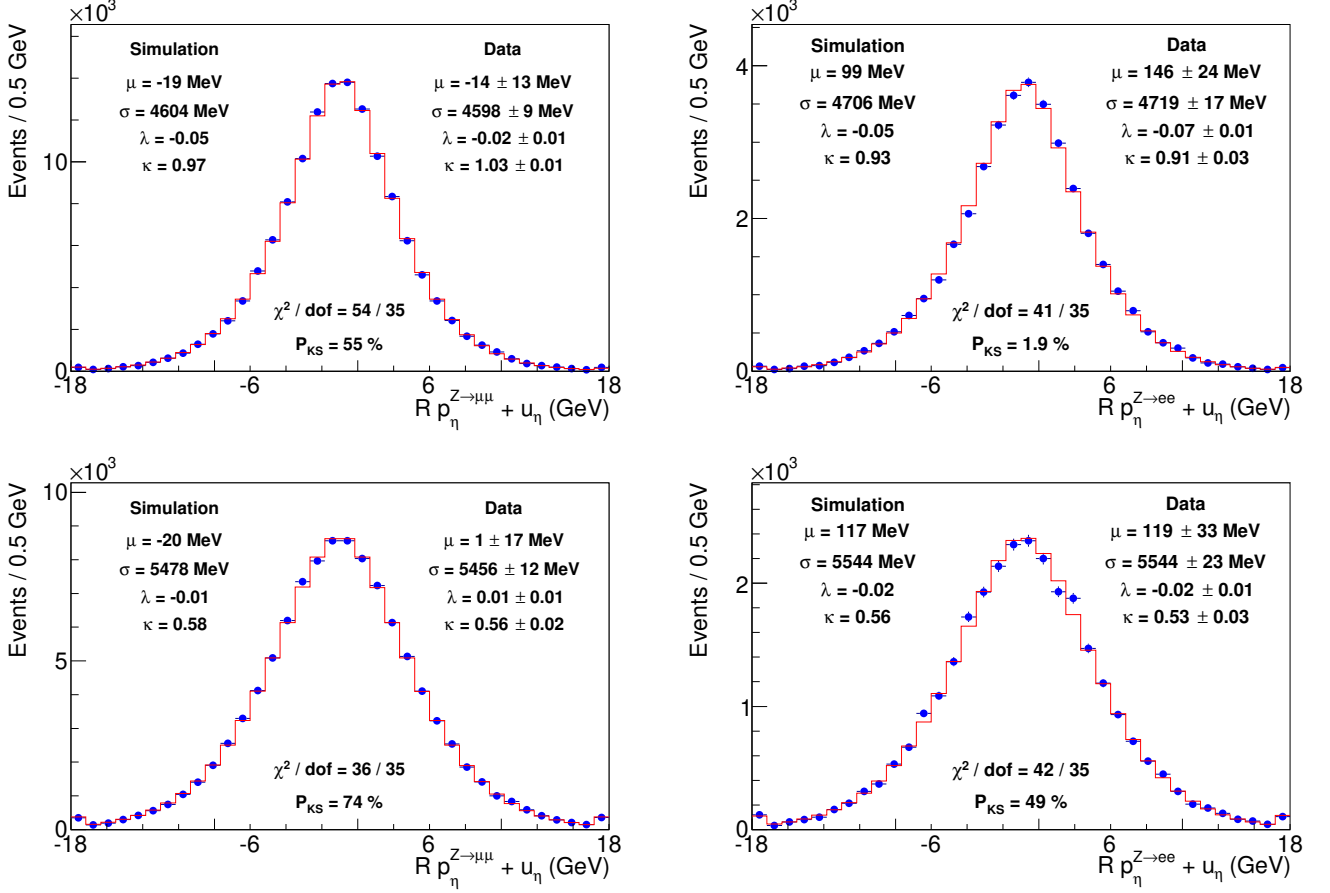
FIG. S25: Distributions of the p_\eta -balance for p_T^{\ell\ell} < 8 GeV (top) and 8 < p_T^{\ell\ell} < 30 GeV (bottom), for the muon (left) and electron (right) channels. The first four moments [mean ( \mu ), rms ( \sigma ), skewness ( \lambda ), and excess kurtosis ( \kappa )] are shown.
