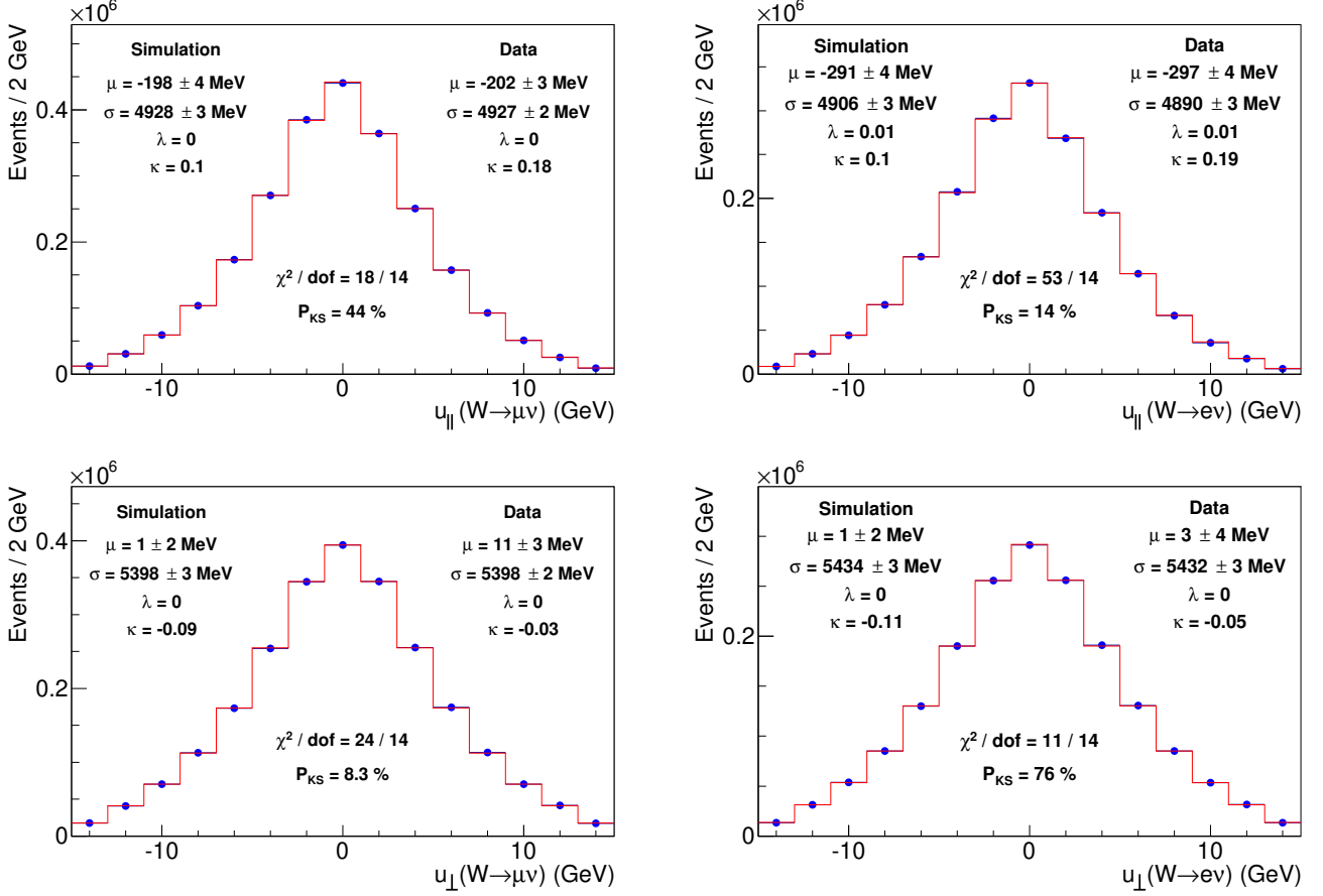
FIG. S31: Distributions of u_{\parallel} (top) and u_{\perp} (bottom) from simulation (histogram) and data (circles) for W boson decays to \mu\nu (left) and e\nu (right) final states. The simulation uses parameters fit from W and Z boson data, and the uncertainty on the simulation is due to the statistical uncertainty on these parameters. The data mean ( \mu ), rms spread ( \sigma ), skewness ( \lambda ), and excess kurtosis ( \kappa ) are well modeled by the simulation. The \chi^2 values and the Kolmogorov-Smirnov (KS) probabilities are based only upon the statistical uncertainties in the data and do not take into account the systematic uncertainties in the simulation.
