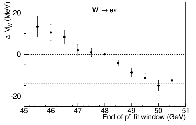
FIG. S41: Variations of the M_W value determined from the neutrino-transverse-momentum fit as a function of the choice of the lower (top) and upper (bottom) edge of the fit range, for the muon (left) and electron (right) channels. Uncertainty bars indicate the expected statistical variation with respect to the default fit range, as computed using pseudoexperiments. The dashed lines indicate the statistical uncertainty from the default mass fit.
