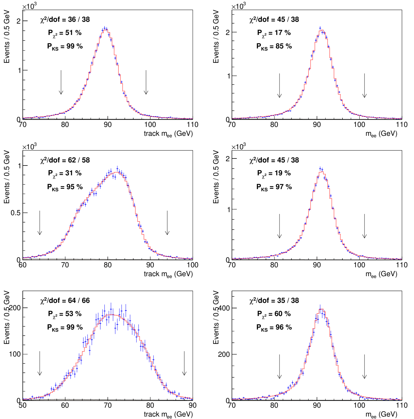
FIG. S16: Distributions (circles) of dielectron mass calculated using (left) only track information and (right) calorimeter E_T with best-fit simulation templates overlaid (histogram) for events with nonradiative electrons (top), one radiative electron (middle), or two radiative electrons (bottom). Fit ranges are enclosed by arrows.
