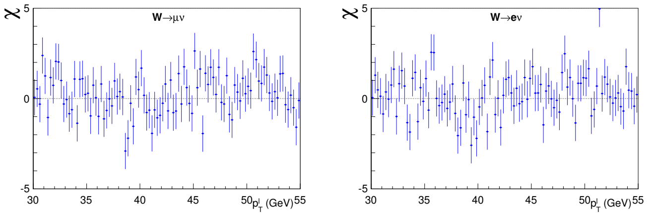
FIG. S37: Differences between the data and simulation, divided by the expected statistical uncertainty, for the p_T^\ell distributions in the muon (left) and electron (right) channels.
