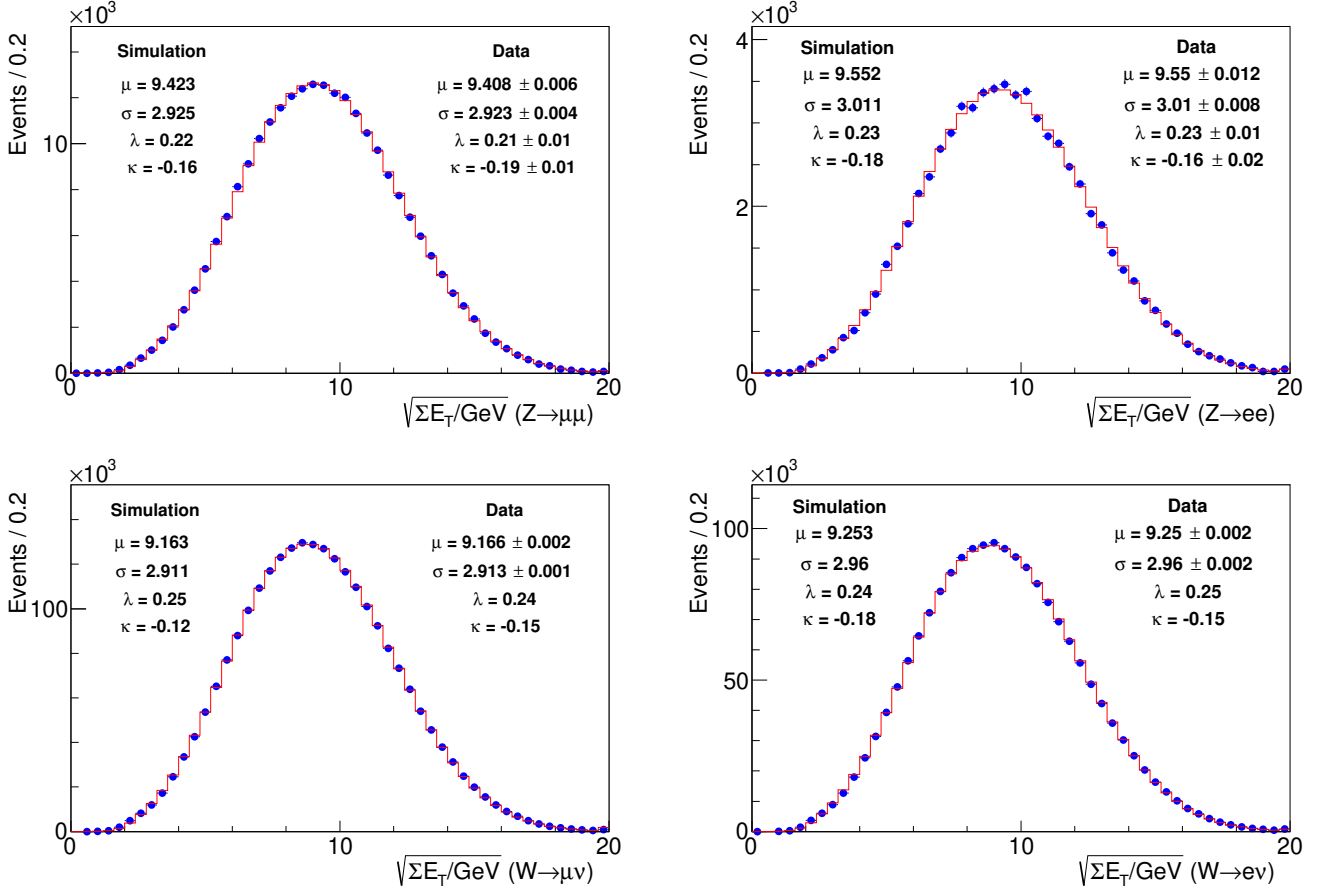
FIG. S29: Distributions of \sqrt{\Sigma E_T} for the muon (left) and electron (right) channels, comparing data (blue points) and simulation (red histogram) for Z (top) and W (bottom) boson candidate events.
