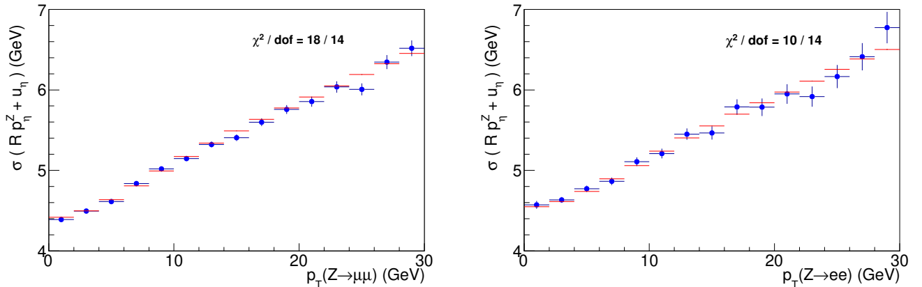
FIG. S24: Resolution on Rp_T^{\ell\ell} + u_\eta in simulated (lines) and experimental (circles) data for Z -boson decays to muons (left) and electrons (right).
