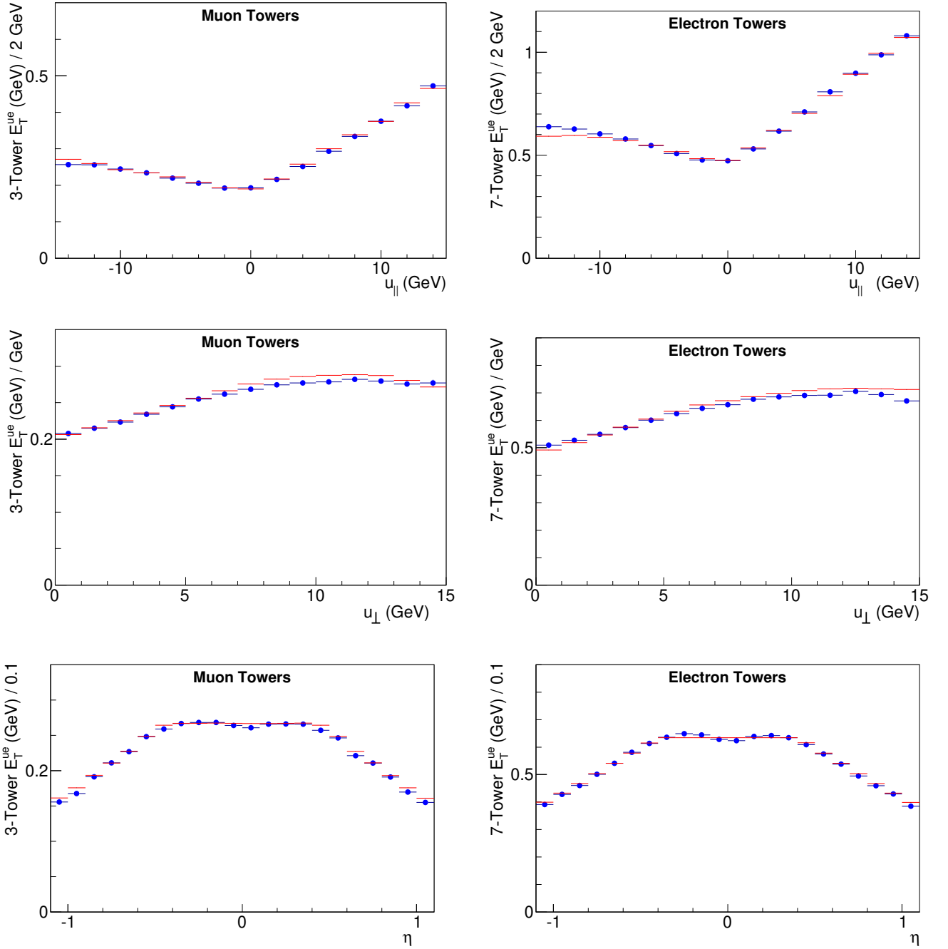
FIG. S20: Variation of hadronic E_T in the three-tower (left) and seven-tower (right) region rotated by 90^\circ in azimuth from the muon (left) or electron (right) as a function of u_{\parallel} (top), |u_{\perp}| (middle), and \eta (bottom) for W \rightarrow \mu\nu (left) or W \rightarrow e\nu (right) data (blue circles) and simulation (red lines).
