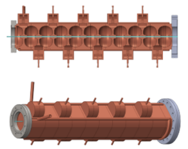
Linac structure
