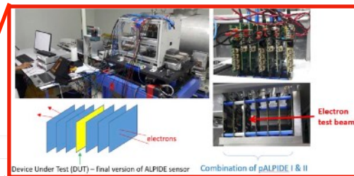
Device Under Test (DUT) - final version of ALPIDE sensor Combination of pALPIDE 1 & II
