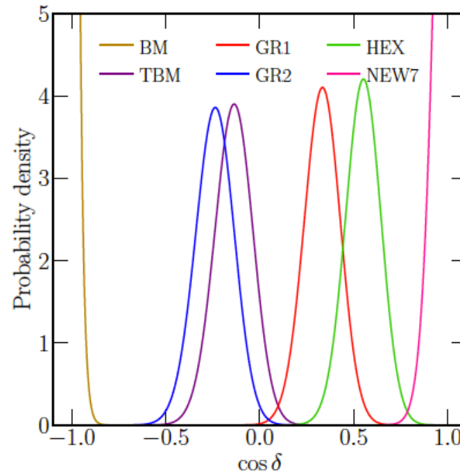
Figure 2: P_{\cos\delta} as a function of \cos\delta for various mixing patterns. Here we have assumed that P_z(z) is a Gaussian centered at the experimental best-fit value of z , with width of 1\sigma .
