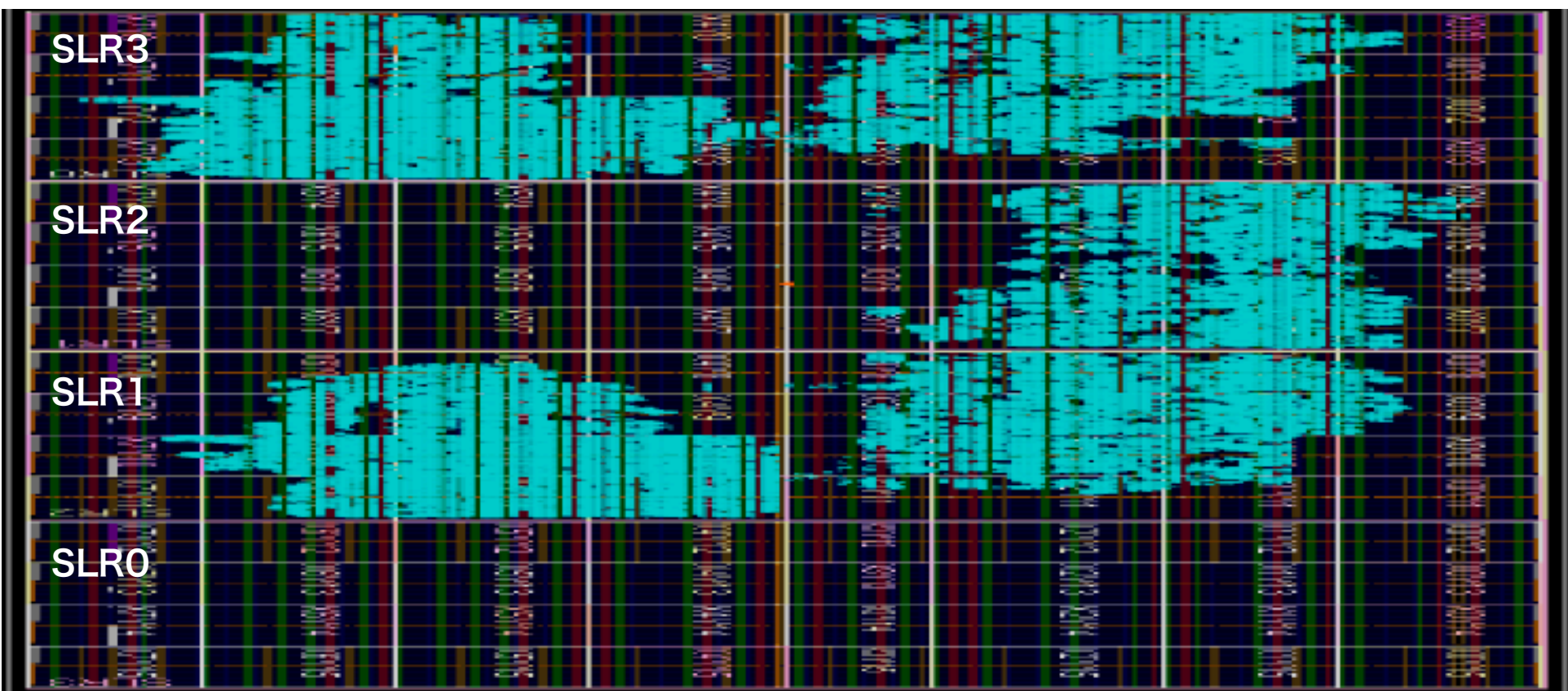
Implementation of the TGC track segment reconstruction in XCVU13P (SLR0 and SLR2 left part reserved for other blocks)
