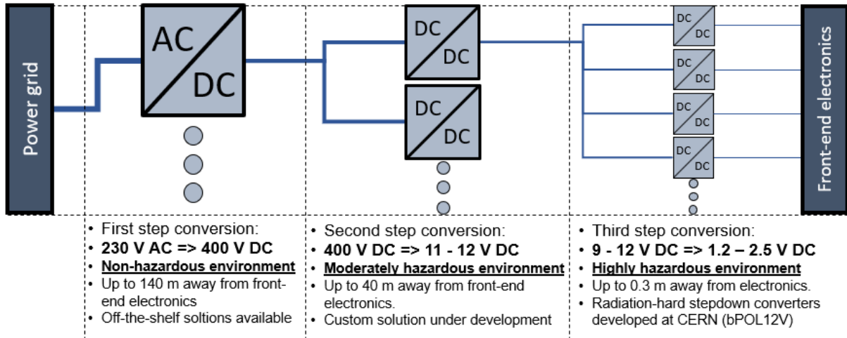
Figure 1: Schematic of the three-stage power conversion chain for the CMS upgrade phase-2.
