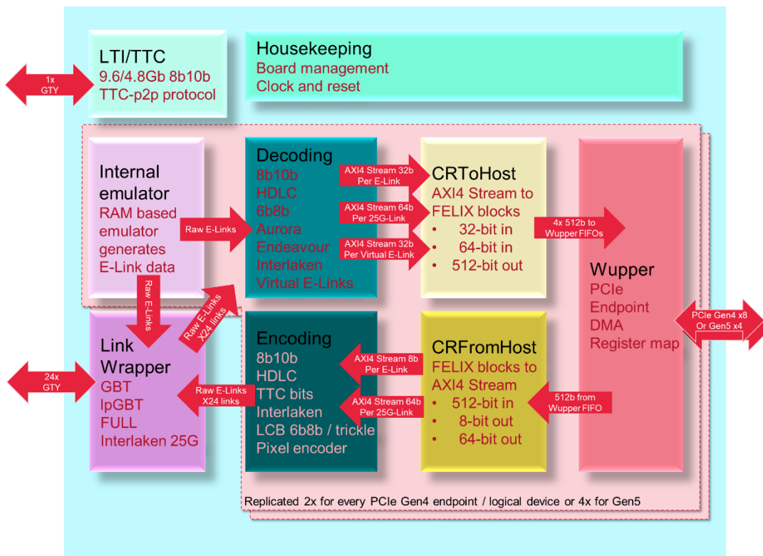
Fig. 2. Run 4 FELIX firmware architecture diagram.
